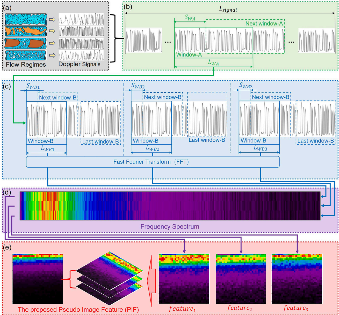
Fig. 3. Illustration of the process of the PIF algorithm for one pseudo-image feature. (a) refers to the flow regime dataset discussed in Section 3. (b), (c), (d), and (e) depict the preprocessing phase in Section 4. (b) refers to the window A process in the PIF algorithm; (c) refers to the window B process in the PIF algorithm. (d) shows the frequency spectrum from the fast Fourier transform. (e) simulates the image form and encodes the pseudo-image feature.
