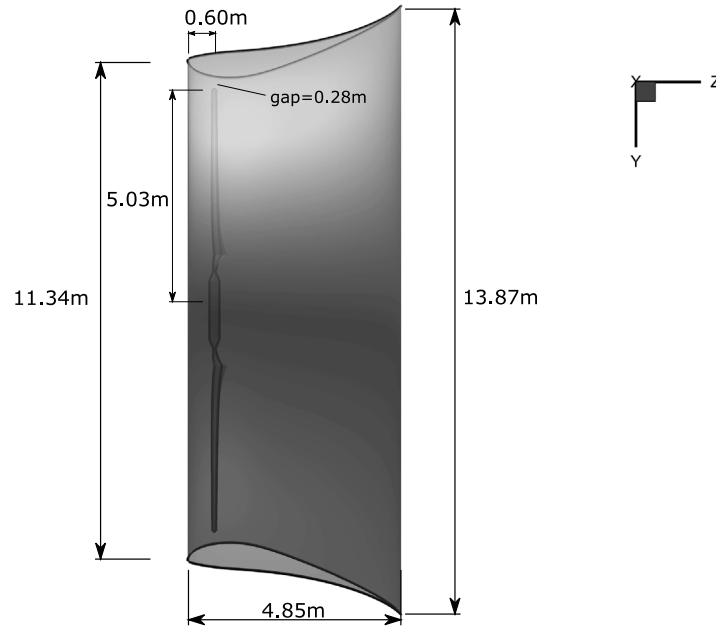
Fig. 2. Dimensions of the shrouded turbine.
