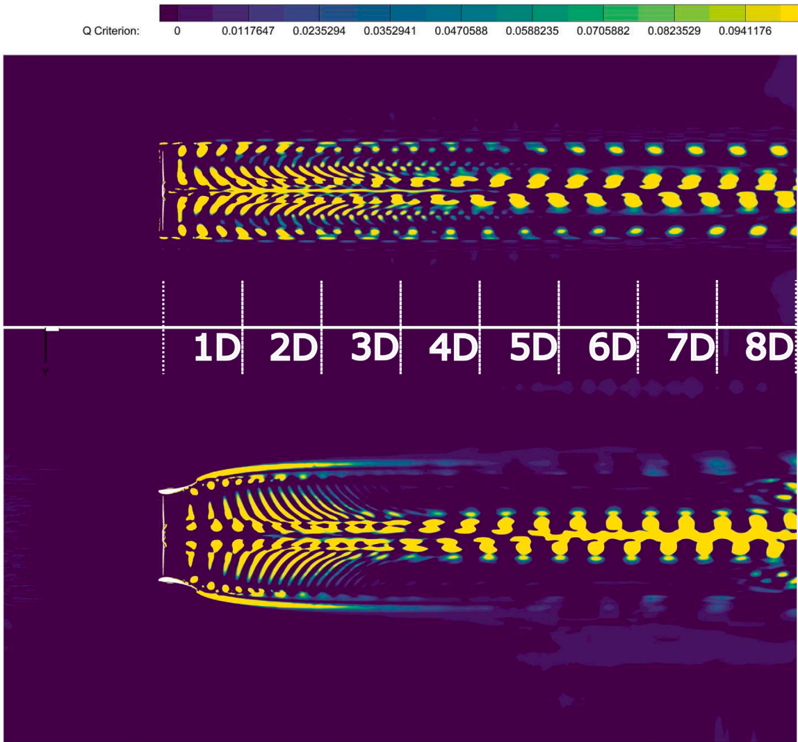
Fig. 4. Contours of q-criteria for the bare turbine (top) and shrouded turbine (bottom) at wind speed equal to 7 ms -1 .
