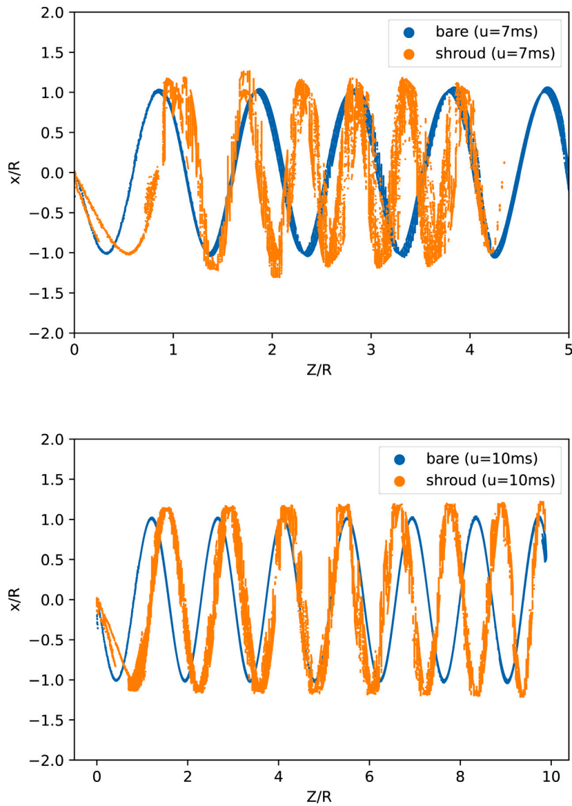
Fig. 8. Planar view of the helical tip vortex development for wind speeds: 7 \text{ ms}^{-1} (top) and 10 \text{ ms}^{-1} (bottom).
