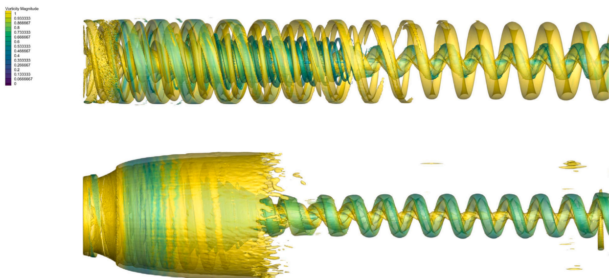
Fig. 6. Comparison of isosurfaces of q-criteria colored by the vorticity magnitude for the bare (top) and shrouded turbine (bottom) at wind speed equal to 7 \text{ ms}^{-1} .
