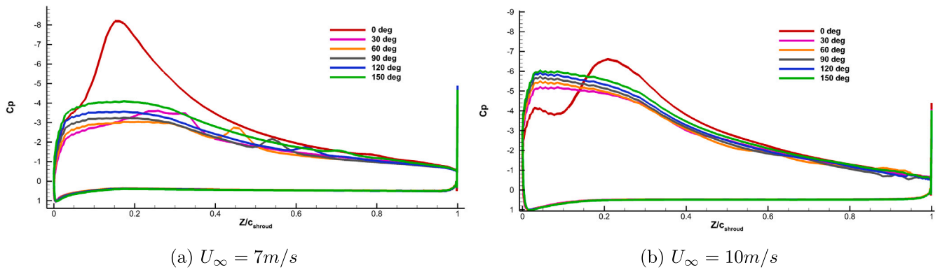
Fig. 11. Pressure coefficient along shroud for several angular slices stations as function of the dimensionless duct-chord coordinate.
