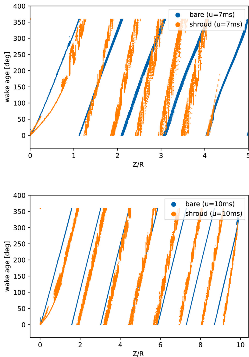
Fig. 9. Tip vortex trajectory in terms of wake age and Z on shrouded and bare turbines for wind speeds: 7 ms -1 (top) and 10 ms -1 (bottom).
