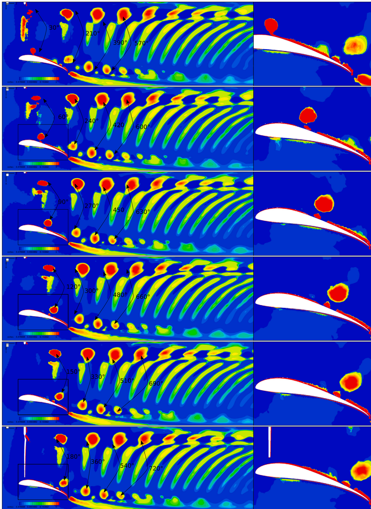
Fig. 10. Contours of q -criteria [ \text{s}^{-1} ] slice of the tip and root vortex age at angular sections at each 30^\circ with shroud vortices interaction in detail.
