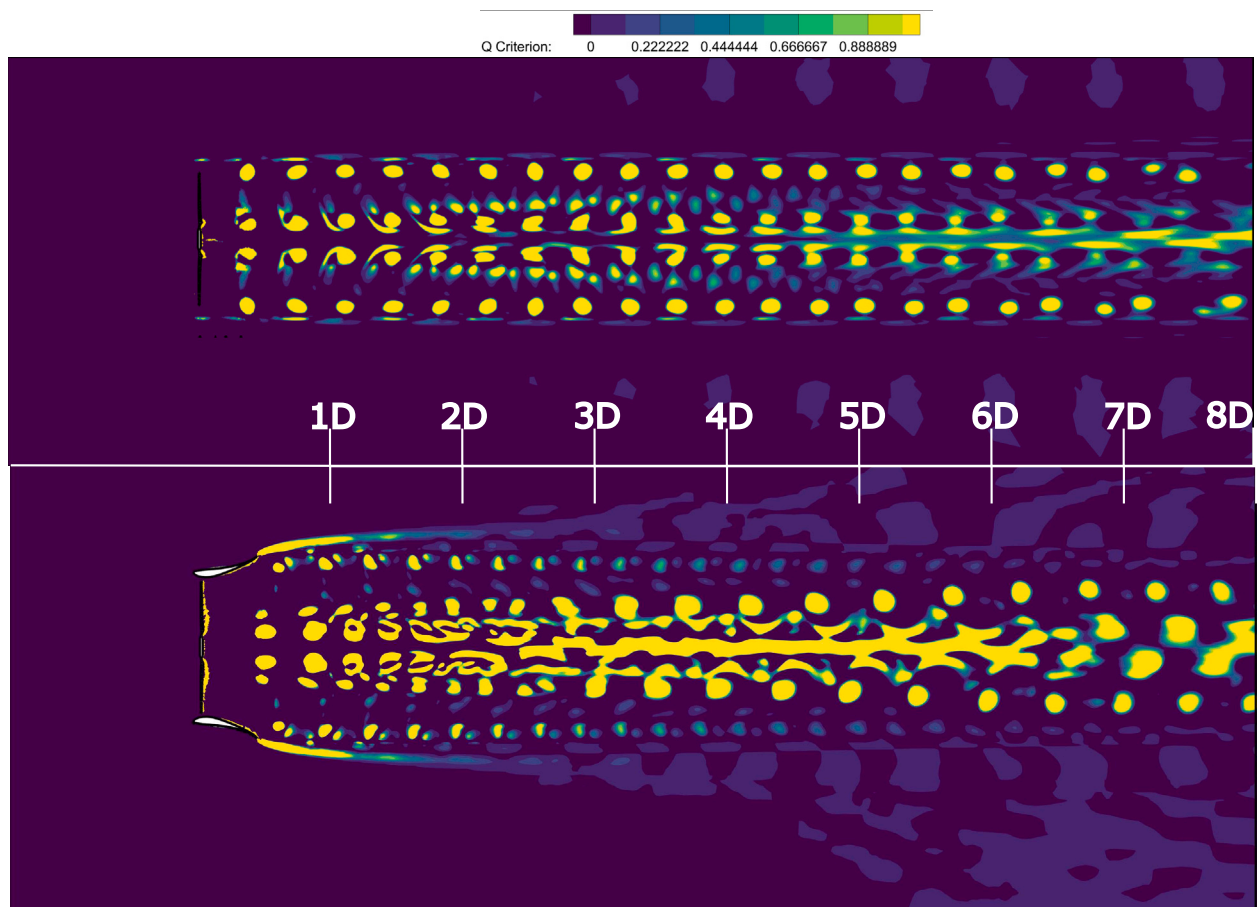
Fig. 5. Contours of q-criteria for the bare turbine (top) and shrouded turbine (bottom) at wind speed equal to 10 \text{ ms}^{-1} .
