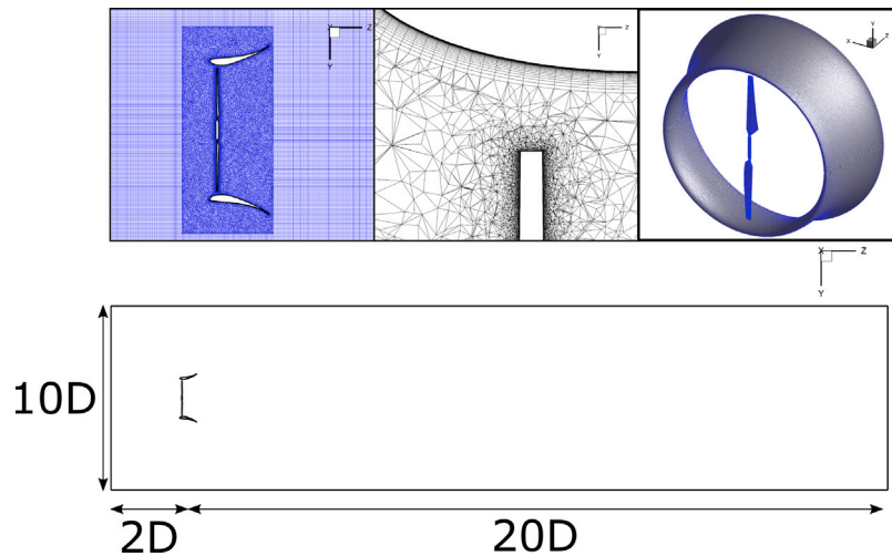
Fig. 1. Schematic of the computational domain (bottom) with details of the mesh refinement around the rotor (top left), tip blade clearance gap (top center) and surface mesh (top right).
