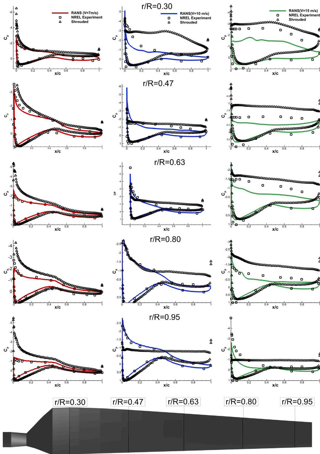
Fig. 3. Numerical and experimental data [56] of pressure coefficient at wind speed ranging from 7 to 15 \text{ms}^{-1} for five radial positions: (a) r/R = 0.3 , (b) r/R = 0.47 (c) r/R = 0.63 (d) r/R = 0.80 and (e) r/R = 0.95 .
