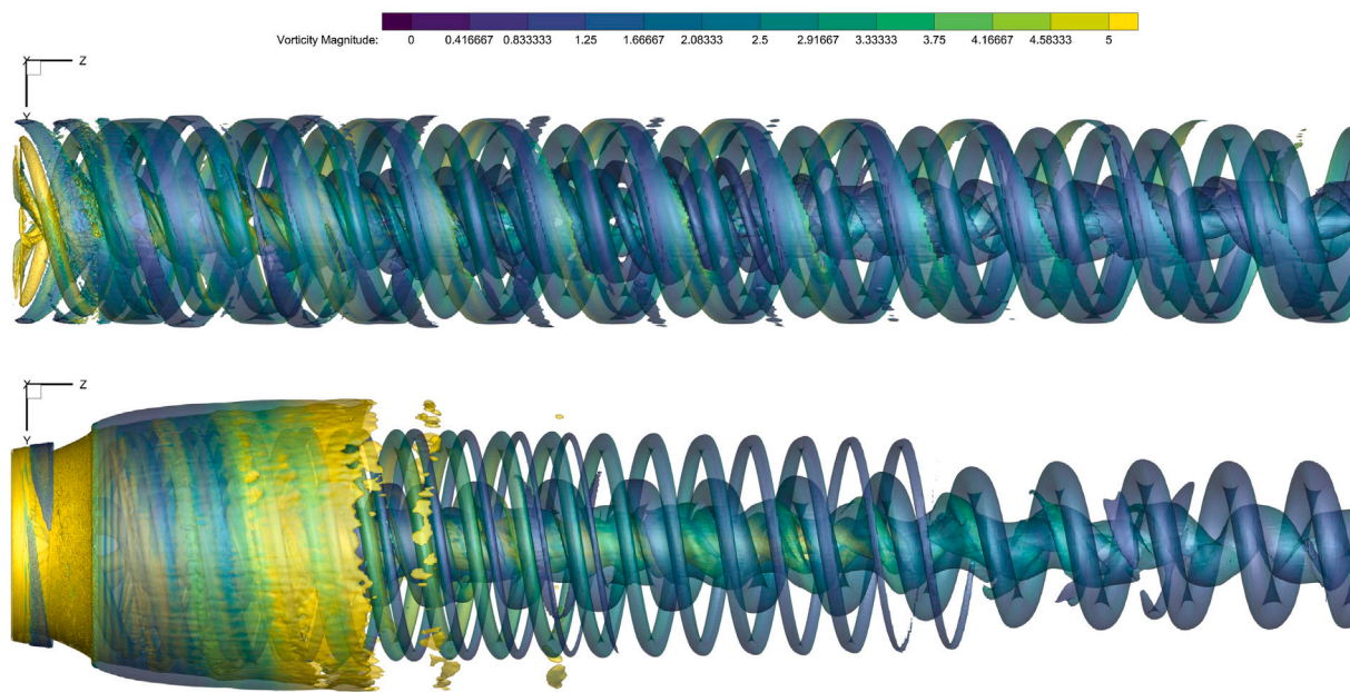
Fig. 7. Comparison of isosurfaces of q -criteria colored by the vorticity magnitude for the bare (top) and shrouded turbine (bottom) at wind speed equal to 10 \text{ ms}^{-1} .
