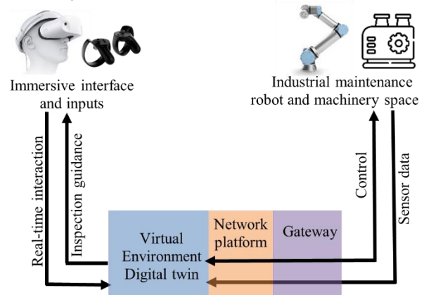
Figure 3: General elements to implement for telepresence maintenance.
