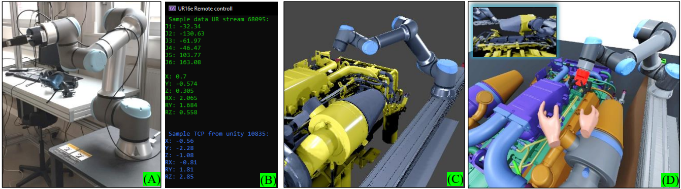
Figure 7: Proposed teleexistence framework for the evaluation of vessel maintenance tasks, (A) physical robot, (B) C# console gateway application, (C) machinery space simulation, and (D) teleexistence user interface.
