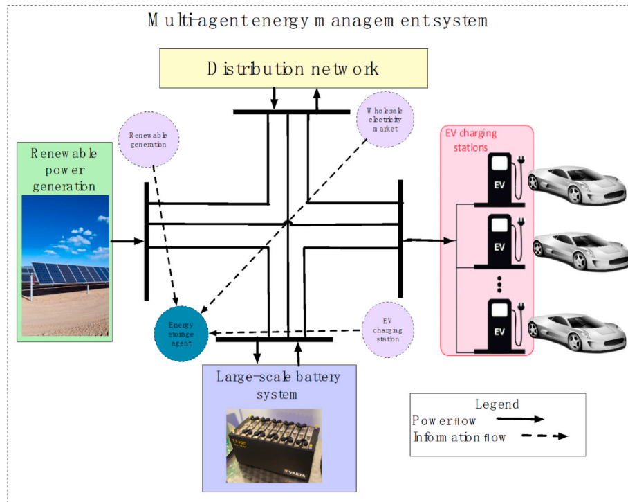
Fig. 1. Power flow and information flow of the distribution network connected with various assets.
