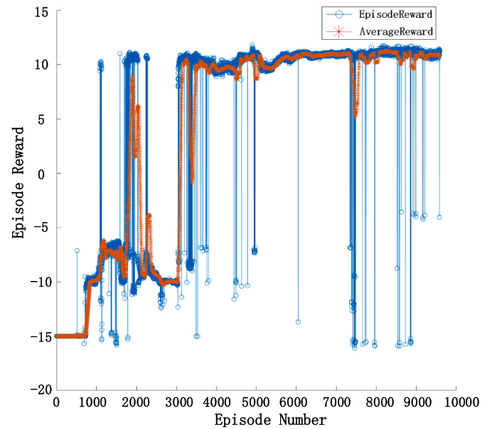
Fig. 13. Reinforcement learning convergence for TD3.
