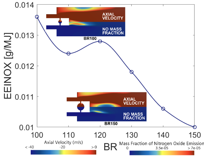
FIGURE 13: NO GENERATION AT \phi = 0.1
