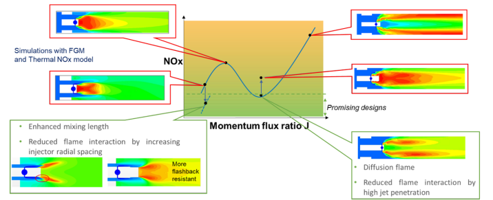
FIGURE 3: MOMENTUM FLUX RATIO EFFECT ON NO_x EMISSIONS [11]
