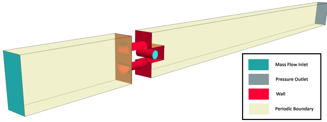
FIGURE 5: COMPUTATIONAL DOMAIN AND BOUNDARY CONDITIONS
