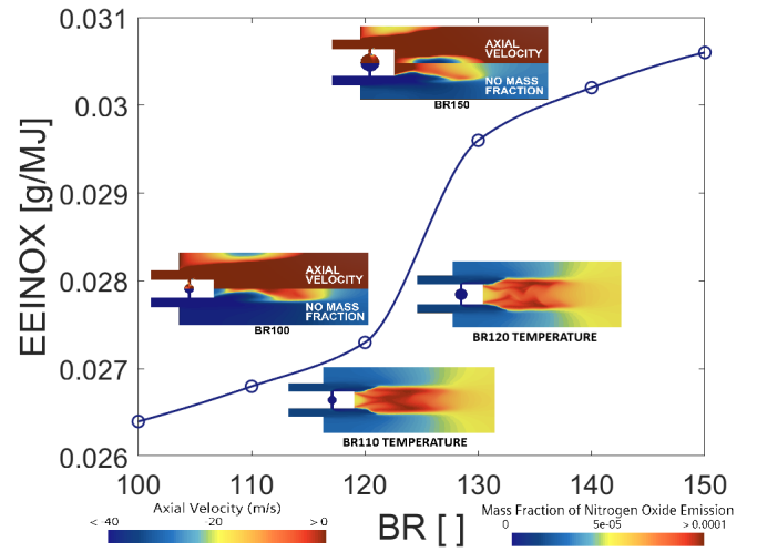
FIGURE 14: NO GENERATION AT \phi = 0.3
