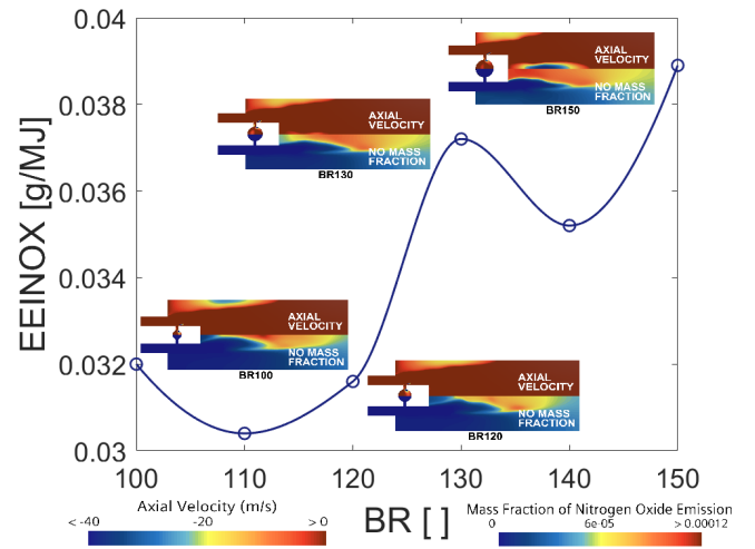
FIGURE 15: NO GENERATION AT \phi = 0.4
