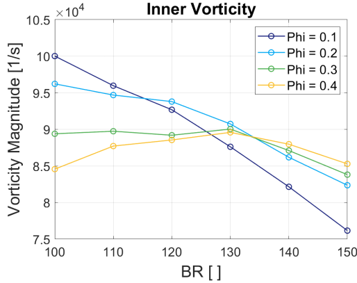
FIGURE 8: VORTICITY IN THE INNER SHEAR LAYER
