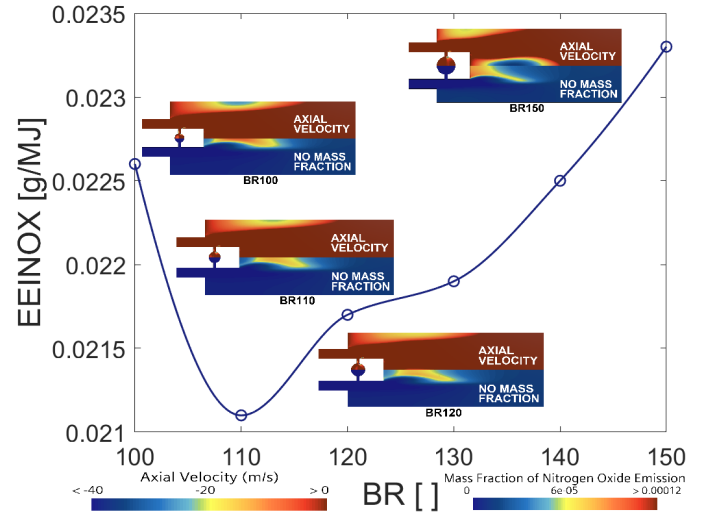
FIGURE 12: NO GENERATION AT \phi = 0.2
