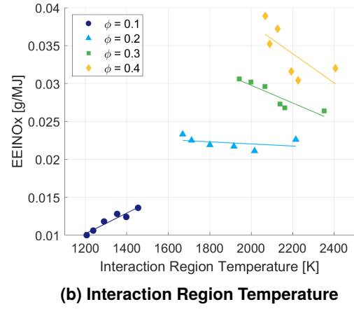
FIGURE 16: NO SENSITIVITY TO IRZ LENGTH AND INTERACTION REGION TEMPERATURE
