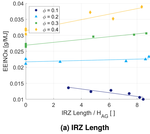
FIGURE 16: NO SENSITIVITY TO IRZ LENGTH AND INTERACTION REGION TEMPERATURE
