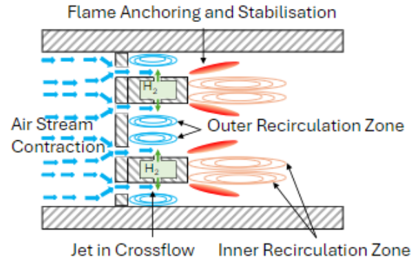
FIGURE 1: HYDROGEN MICROMIX CONCEPT [11]
