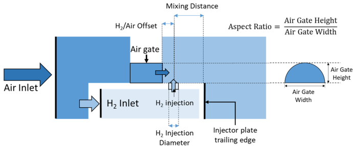
FIGURE 2: HYDROGEN MICROMIX DESIGN SPACE [11].
