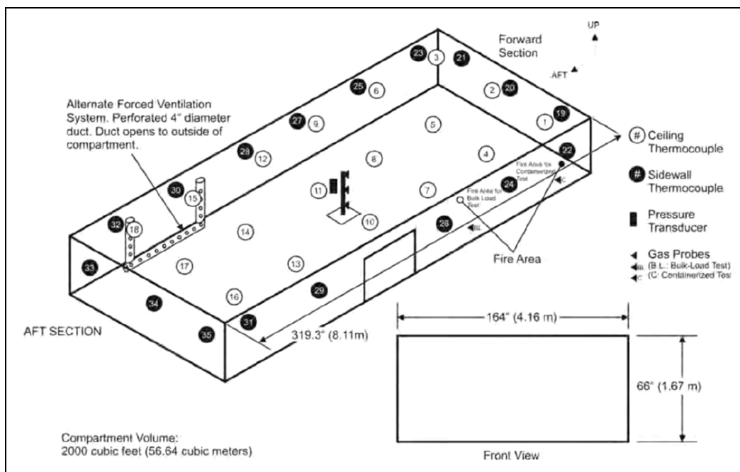
Figure 1. Cargo compartment layout and instrumentation locations.
