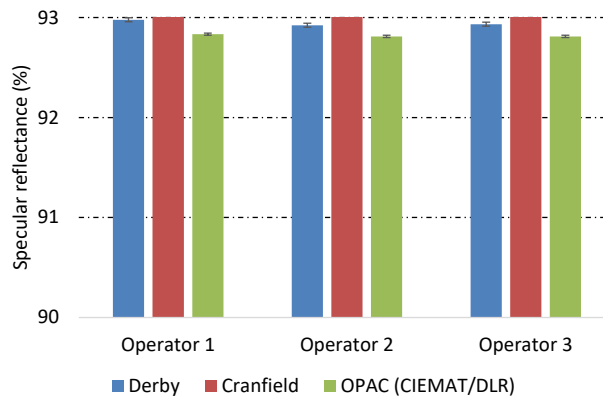
Figure 4. Solar weighted specular reflectance of clean silvered glass mirror using three different Condors
