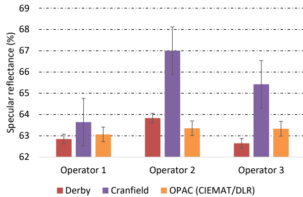
Figure 6. Solar weighted specular reflectance of soiled silvered-glass mirror using three different condors
