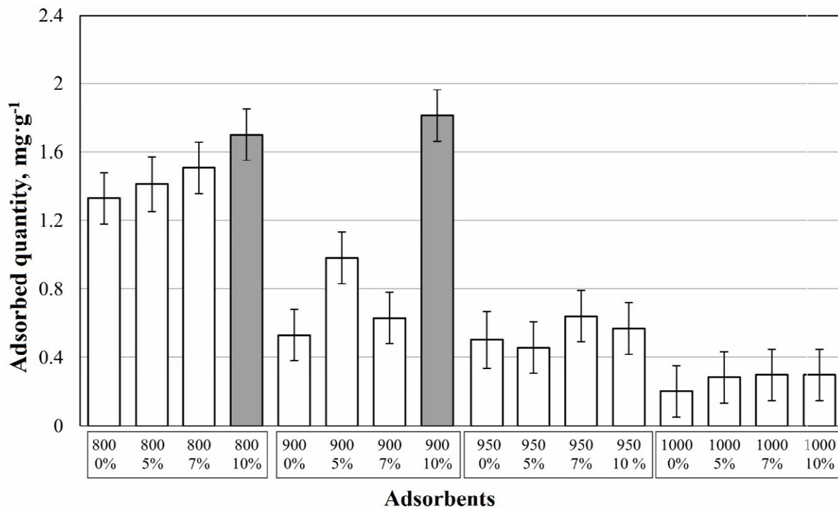
Fig. 4. Preliminary adsorption test of different prepared materials.
