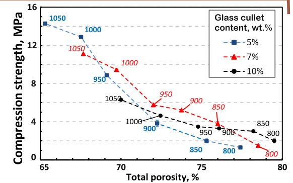
Dependence of the compression strength on the firing temperature and porosity
