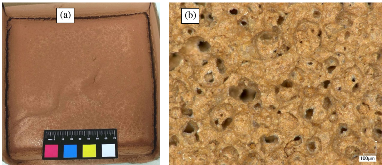
Fig. 1. CF with 7 wt.% MC content. a) green sample after drying; b) fired at 900°C, optical microscope at magnification X200 times.
