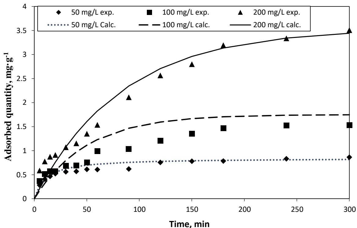
Fig. 9. The adsorption amount of dye onto MC10-900 obtained experimentally and fitted pseudo-second order kinetic model.
