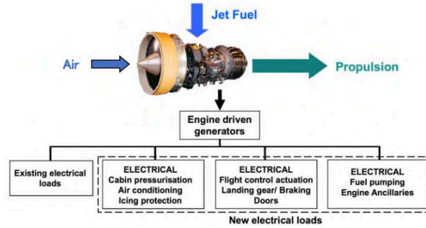
Fig. 6 No-bleed engine architecture of the MEA [5]
