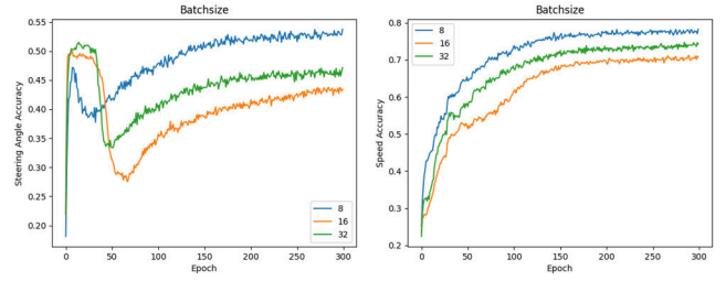
Fig. 2. Batch-size comparison (steering angle and speed accuracy)
