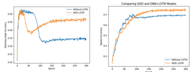
Fig. 8. Comparison of DNN and DNN+LSTM models
