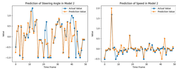
Fig. 11. Comparison of Actual and Predicted Values for Model 2
