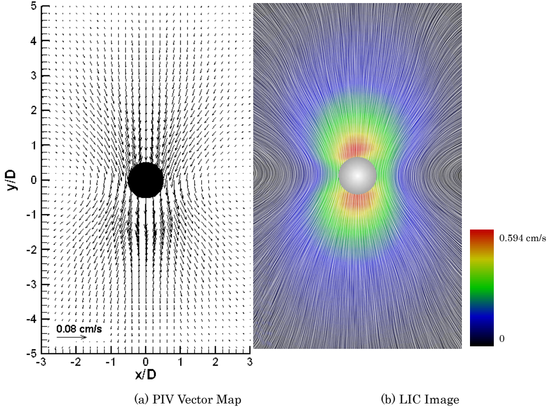
Fig. 2 Data from Newtonian Fluid (6.35mm metal ball, 1 diameter from wall)
