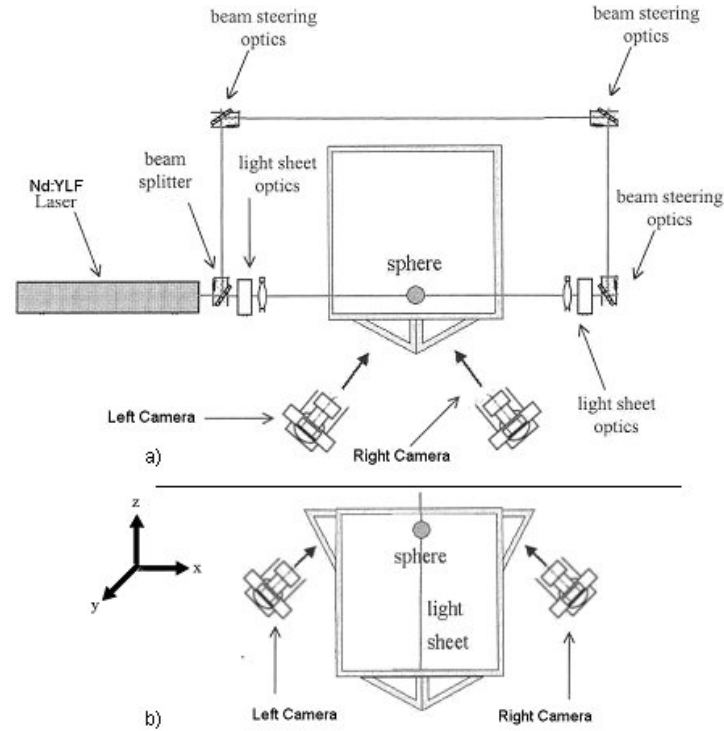
(a) Parallel wall measurements (b) Perpendicular wall measurements
