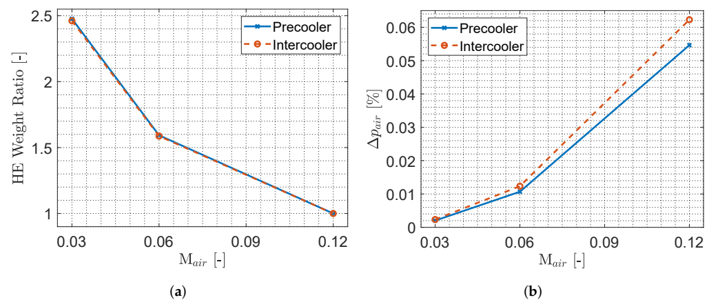
Figure 16. Pre-cooler and inter-cooler HE: (a) the weight ratio of HE, and (b) air-side pressure drop percentage across the HE tubes (associated with the effectiveness of \epsilon = 0.6 and inlet velocity of V_{LH_2} = 150 [m/s] at the design point of HE) for varying air-side Mach number.
