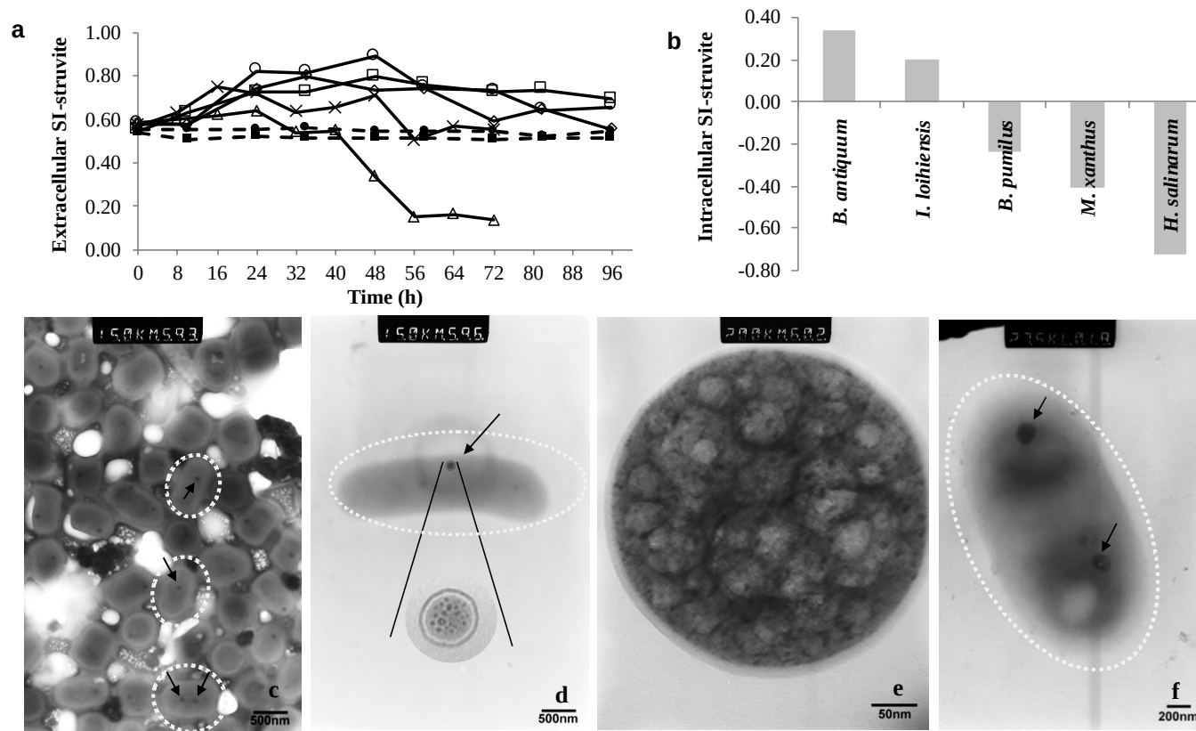
385 Fig. 4 Variation of extracellular SI struvite (a) in microbial cultures of H. salinarum (×), B. pumilus (◇), M. xanthus (○), B. antiquum (Δ) and 386 I. loihiensis (□), and the microbial intracellular SI struvite (b) during the 72/96 h incubation time. TEM pictures shows (c) an overview of B. 387 antiquum culture (60 h), cells (white dotted circles) containing one or two electron-dense structures (black arrows); (d) a vesicle-like 388 structure (black arrow) inside B. antiquum cell (white dotted circles), with intact membrane structure, and occupied with electron dense 389 clustered granules, as shown in an enlarged (8-time) version; (e) detail of the vesicle, whose internal structures were destroyed by a high-
