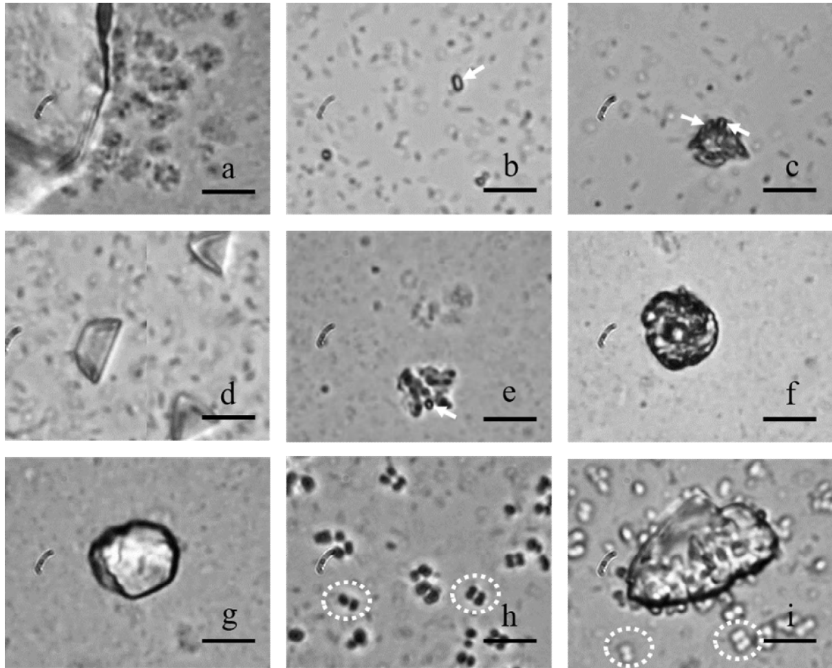
Fig. 2 Optical microscope photograph observed in late exponential phase of growth (16–24 h): (a) cell clusters of I. loihiensis around crystal surface, (b) small particles (white arrow) about 1 µm in M. xanthus culture, (c) aggregate of small particles (white arrows) in B. antiquum culture, (d) triangle and trapezoidal crystals in M. xanthus culture, (e-g) a morphology evolution in I. loihiensis culture: from (e) aggregate of cell clusters and particles (white arrow) to (f) large particle (approx. 5 µm) with clear boundary, and to (g) large particle (approx. 5 µm) of crystalline structure view. (h) Crusted two-cell or tetrad cell clusters in B. pumilus culture, and (i) their aggregate onto crystal surface (white dotted circle - crusted cell cluster). Bar scale - 4.06 µm.
