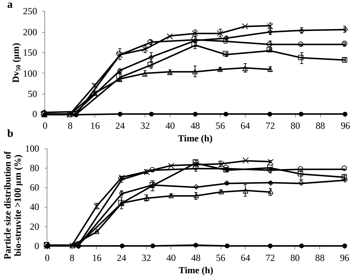
Fig. 5 Variation of D_{v50} (a) and cumulative volume percentage of crystal \geq 100 \mu\text{m} (b) in synthetic solution over incubation period, in the presence of H. salinarum (x), B. antiquum ( \Delta ), B. pumilus ( \diamond ), M. xanthus ( \circ ) and I. loihiensis ( \square ) and in non-inoculated controls ( \bullet ). Error bars indicate standard deviation of duplicates. D_{v50} is the value of particle diameter at 50% in the cumulative particle size distribution on a volume basis.
