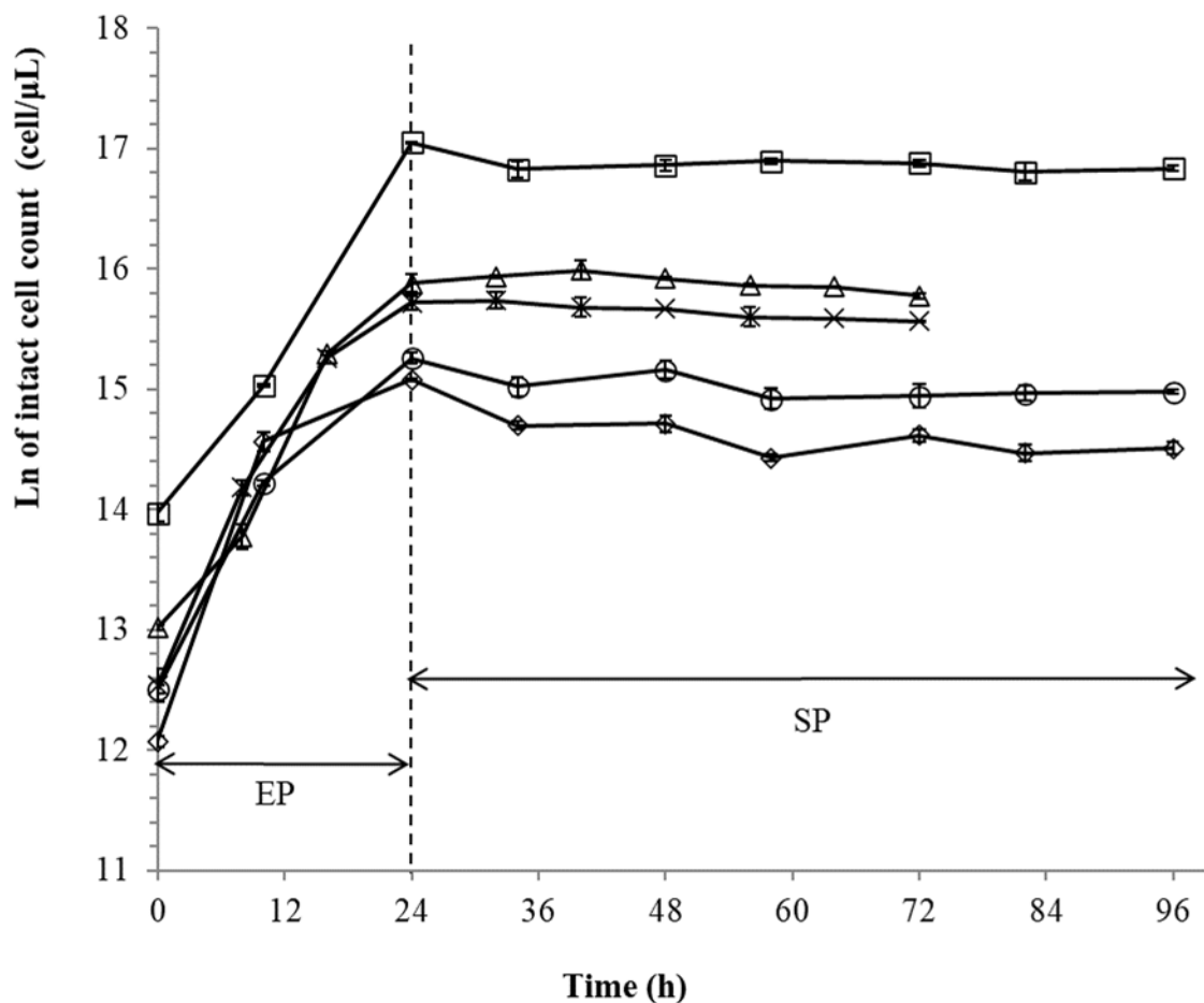
Fig. 1. Natural logarithm of intact cell count of H. salinarum (×), B. antiquum (Δ), B. pumilus (◇), M. xanthus (○) and I. loihiensis (□) over the incubation period. Error bars indicate standard deviation of duplicates. (EP - exponential phase, SP - stationary phase of growth)
