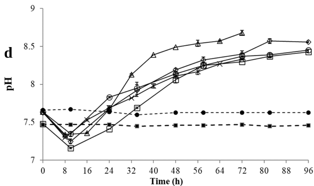
Fig. 3 Variation of (a) PO 4 -P, (b) Mg 2+ , (c) NH 4 -N and (d) pH in microbial cultures of H. salinarum (×), B. antiquum (Δ), B. pumilus (◇), M. xanthus (○) and I. loihiensis (□) and in non-inoculated controls (●) and (■) during 72/96 h incubation time. Error bars indicate standard deviation of duplicates.
