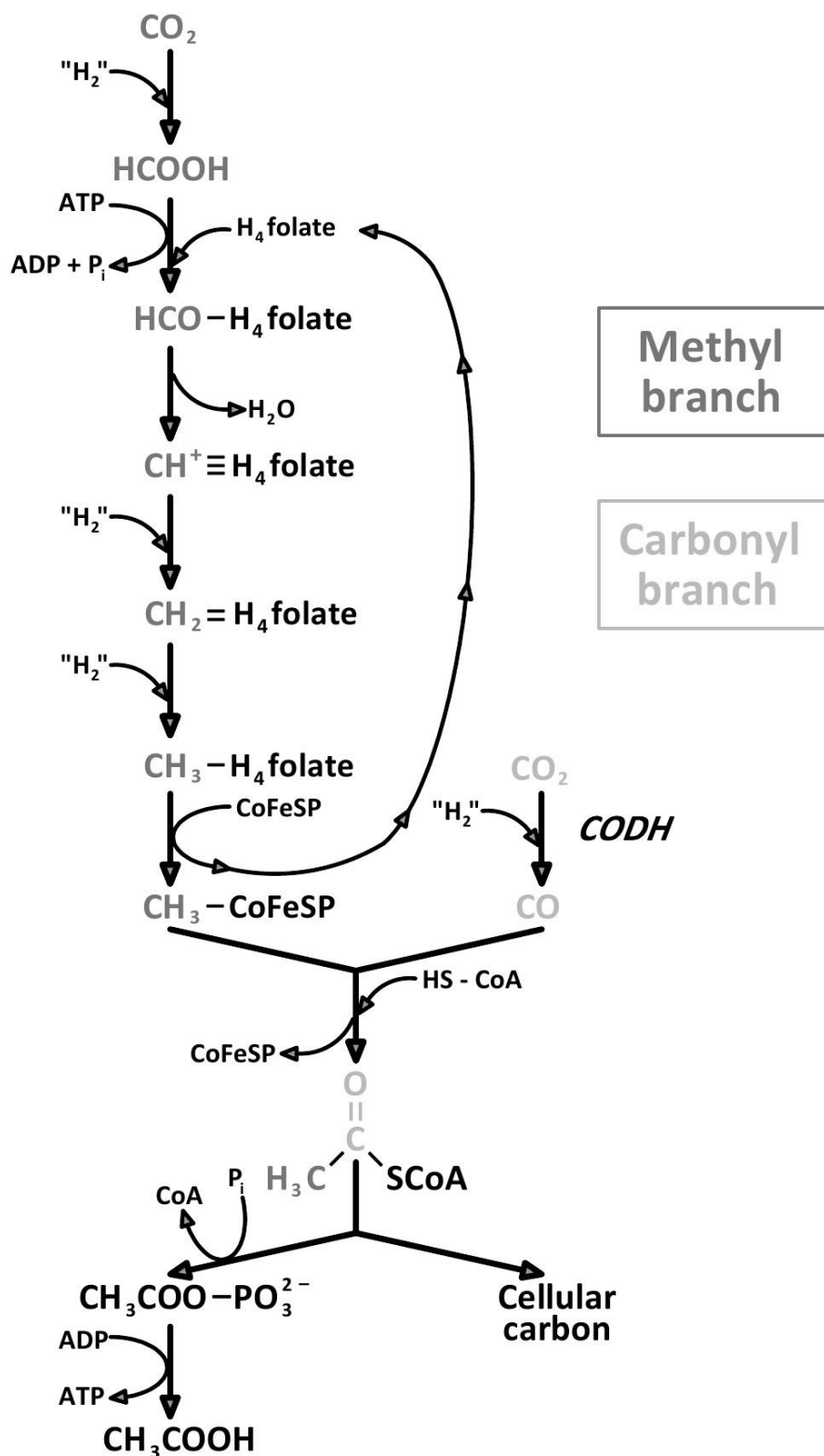
Fig. 5. Wood-Ljungdahl pathway for homoacetogenic acetogenesis. “H 2 ” is used to represent requirement of two electrons and two protons. Adapted from Ragsdale and Pierce, (2008).
