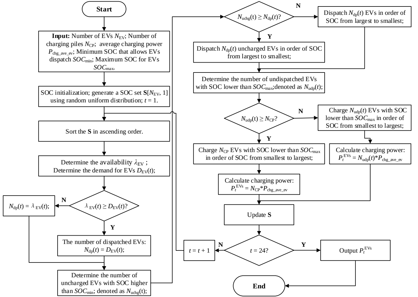
Fig. 7 Flow chart of EVs charging profile modelling
