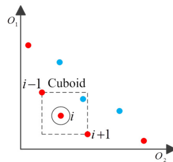
Fig. 2 Computation of the crowding distance [4]
