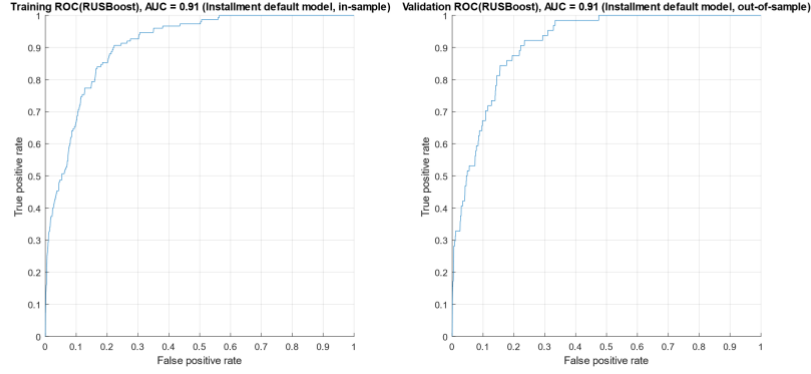
Fig. 2. AUC results for training and validation bank 2
