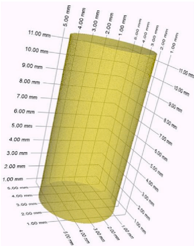
Fig. 4. Micro-CT results in the gauge section of a specimen illustrating 3D rendering of the sample with 60% transparency showing no porosity.
