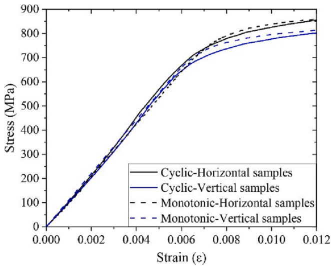
Fig. 9. A comparison of the cyclic and monotonic stress-strain curves.
