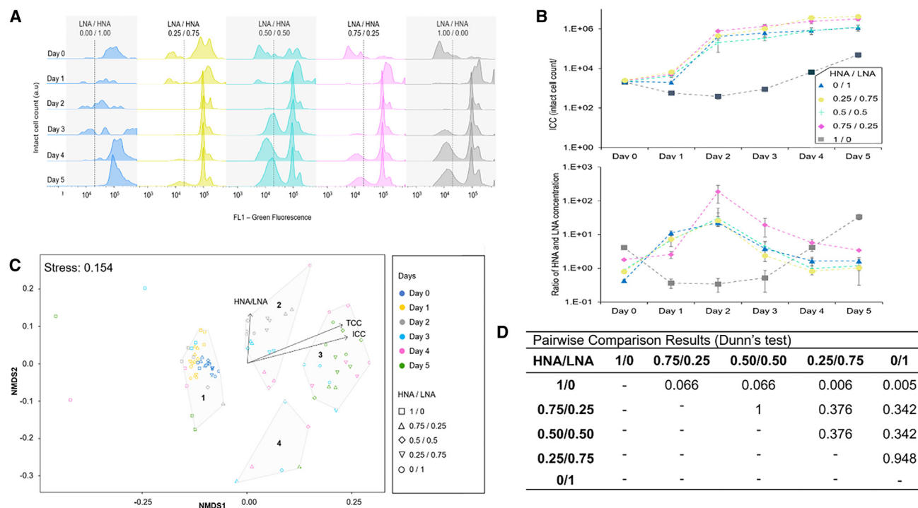
Figure 4. Daily intact cell growth and HNA/LNA ratios: experimental trends and multivariate analyses
