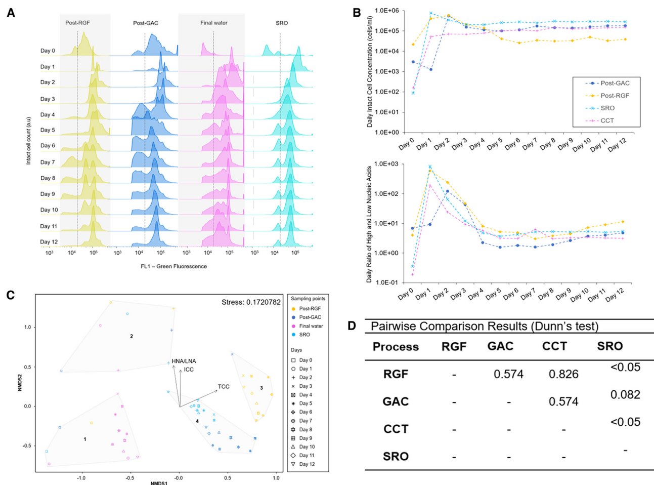
Figure 5. Experimental measurements of the daily cell growth of water coming from different stages of a water treatment works (WTWs) (A) The sample points post-rapid gravity filter (RGF), post-granular activated carbon (GAC), post-chlorine contact tank (CCT) and a service reservoir outlet (SRO) the daily fluorescence fingerprint of each sample. The intact cell count (ICC) variation on the y axis scaled for each sample to visualize the bacterial communities and their fluorescence. (B) The daily variation of the ICC (top) and high and low nucleic acid ratio (HNA/LNA) (lower). (C) NMDS plot obtained from a fingerprint analysis to evaluate the dissimilarities and similarities between and within the samples. The environmental vectors (ICC, HNA/LNA ratio) were included to determine the factors influencing the dissimilarities, 2D stress is indicated. (D) Pairwise comparison results to compare fingerprints between the different source waters after nutrient additional and regrowth experiment. A single replicate's fluorescence fingerprint is shown in (A), cell concentration and HNA/LNA ratio data represent mean values of repeats, with error bars indicating mean concentration errors A and mean HNA/LNA errors in (B).
