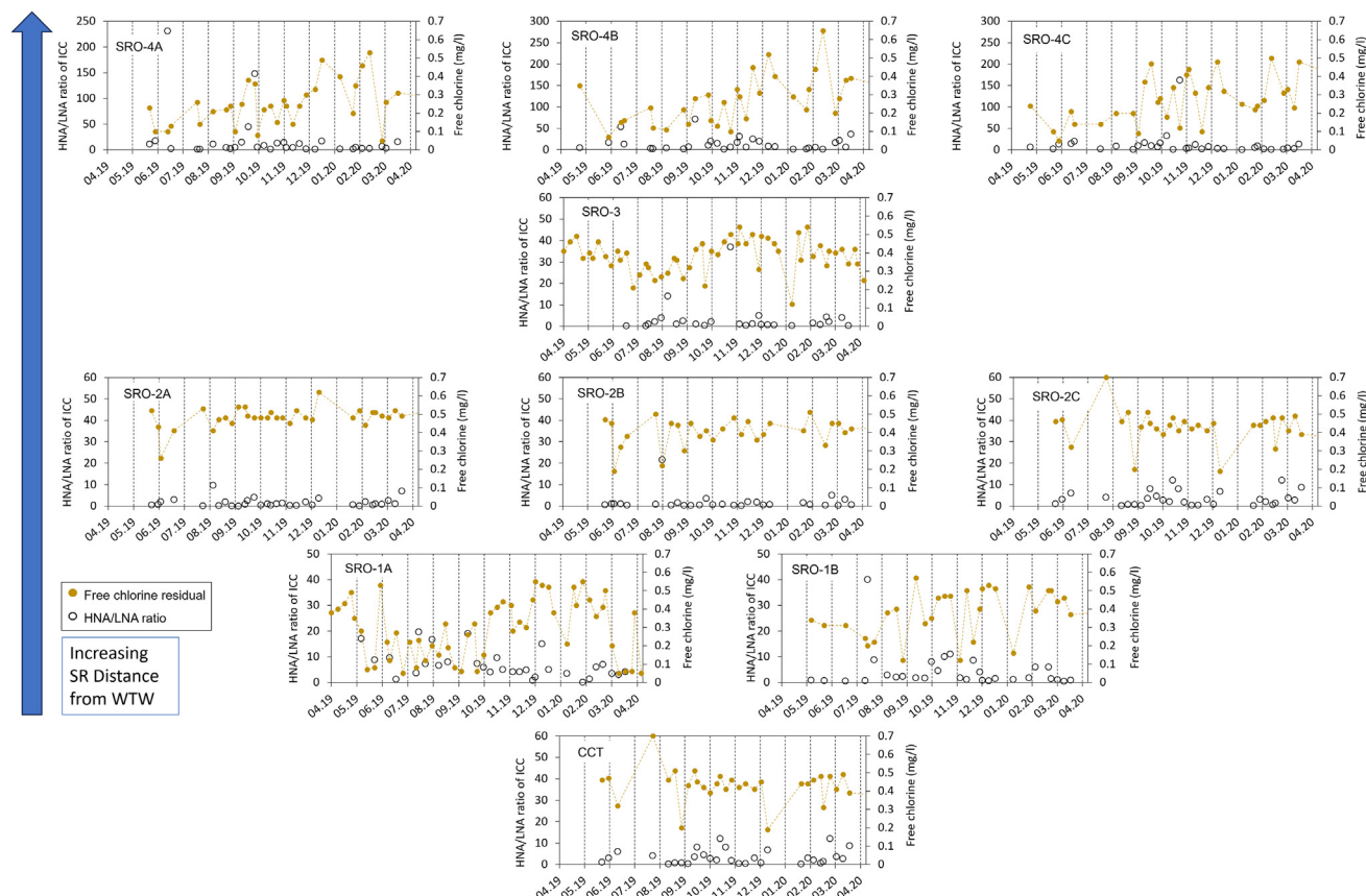
Figure 3. Ratio of high nucleic acid (HNA) and low nucleic acid (LNA) content (HNA/LNA) of intact cell counts (ICCs) and residual chlorine levels from the service reservoir (SR) measured at the SR outlets (SRO) and the chlorine contact tank (CCT) supplying them
