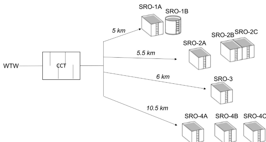
Figure 1. Schematic of the water distribution system, showing the path from a water treatment works (WTW) to various service reservoirs outlets (SROs) within the drinking water distribution systems (DWDS)
