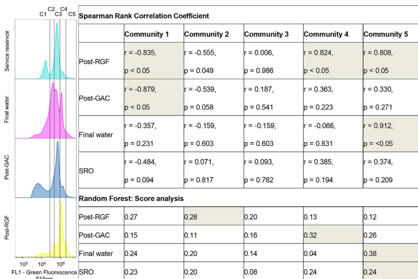
Figure 6. Fingerprint of each water at the end of the regrowth experiment
