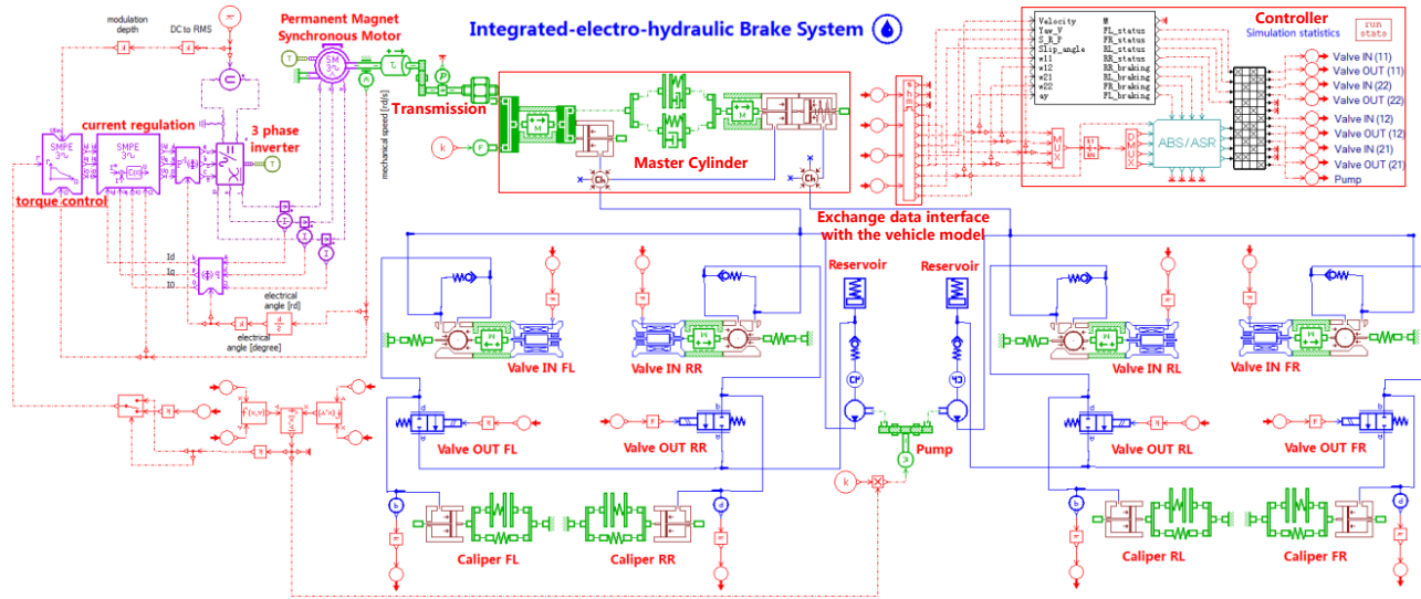
Fig.4. I-EHB actuator simulation model.
