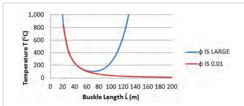
Fig.7. Relationship between temperature and buckle length with different coefficients of friction.
