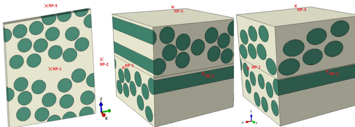
Figure 4: Points related to the RVE faces, were displacement input and reaction load output was controlled
