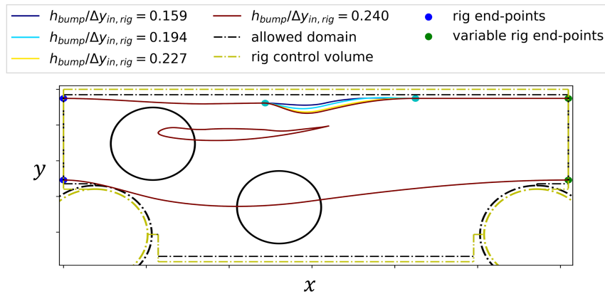
Fig. 11 Schematic of the rig configuration at diversion windmilling and bump geometries used to control the mass flow split between upper and lower channel
