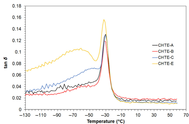
FIGURE 8 Tan \delta curves for samples CHTE-A (black line), CHTE-B (red line), CHTE-C (blue line), and CHTE-E (yellow line). DMA thermograms for samples CHTT, CHTH, CHTP, and CHTD are reported in Figures S16–S19.
