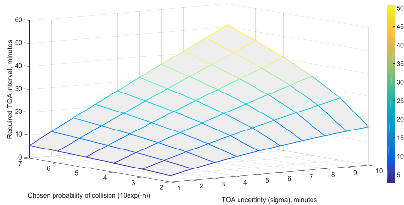
Figure 8. Required TOA interval for different collision probabilities and TOA standard deviation for the involved A/C
