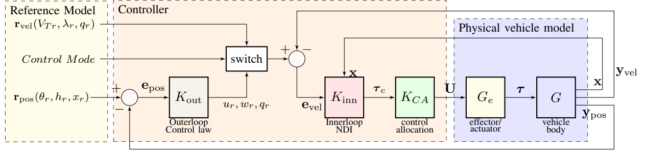
Fig. 1: Control Architecture
