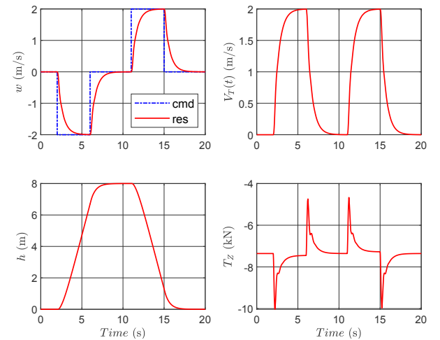
Fig. 3: Vertical Climb and Descent Manoeuvre
