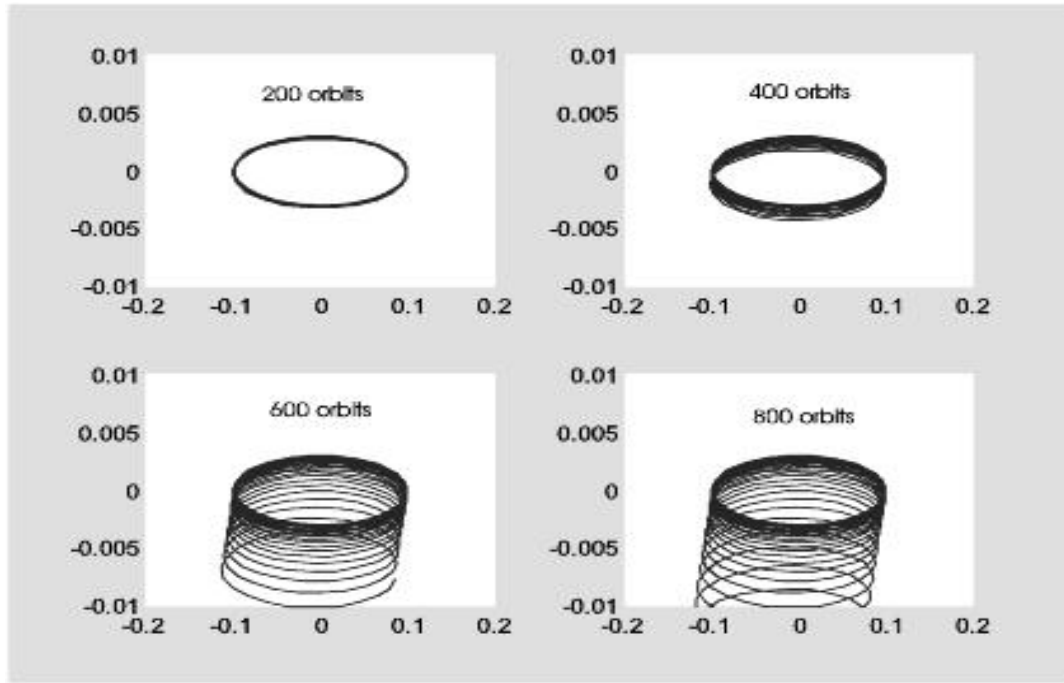
Figure 2: Instability rise in the relative position of the uncontrolled leader-follower formation, y, x plot. The plot was done by using Floquet analysis. It would not be possible to get the same result by direct numerical integration as the algorithm would be unstable after 150 orbits.
