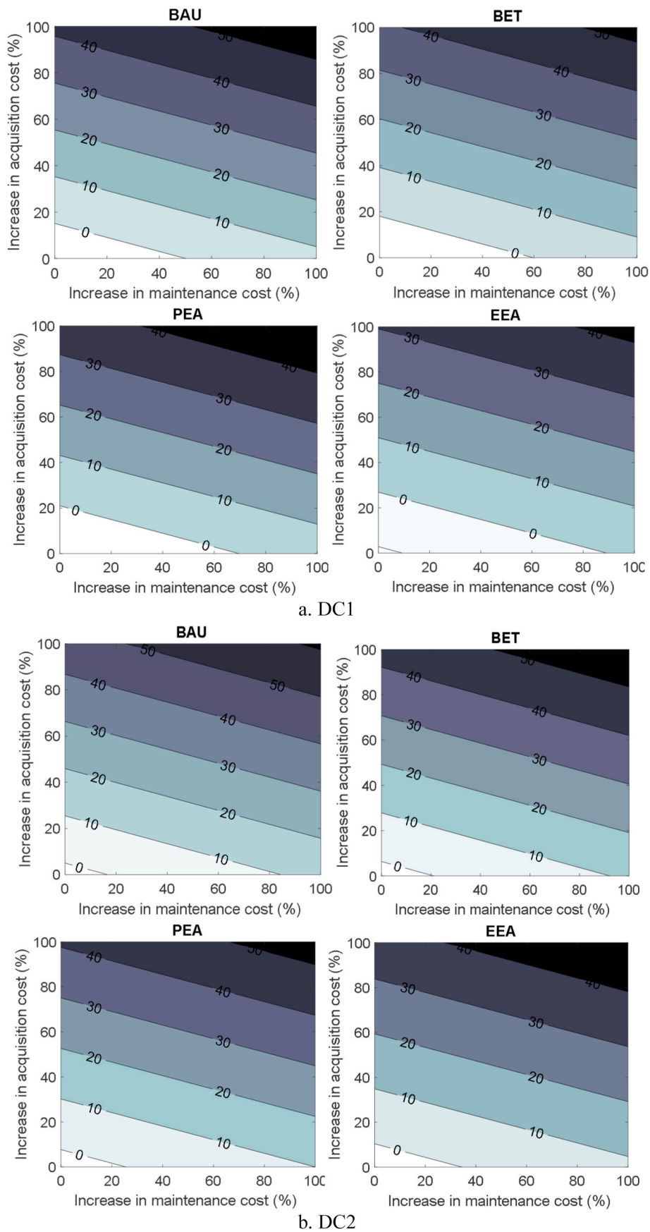
Fig. 20. Direct Operating cost for baseline and HEA optimal design.
