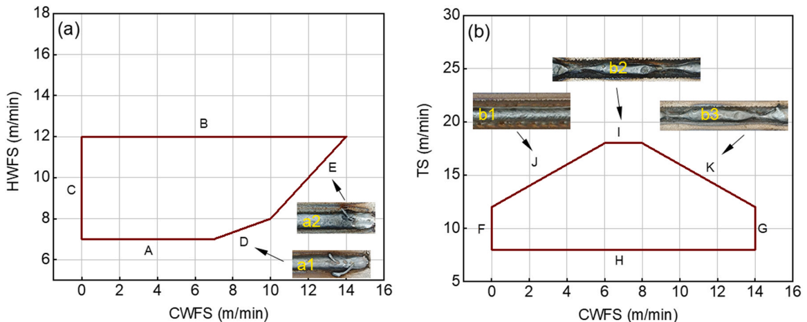
Fig. 11. Working envelope of the CW-GMA process based on bead-on-plate experiments: (a) HWSF vs CWFS, and (b) TS vs CWFS.
