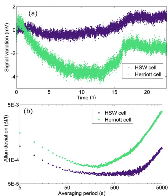
Fig. 10. (a) Mean pulse amplitude variation data for HSW and Herriott cells and (b) the Allan–Werle deviation of this data.
