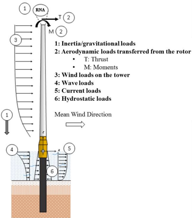
180 Figure 3. Loads on the support structure
