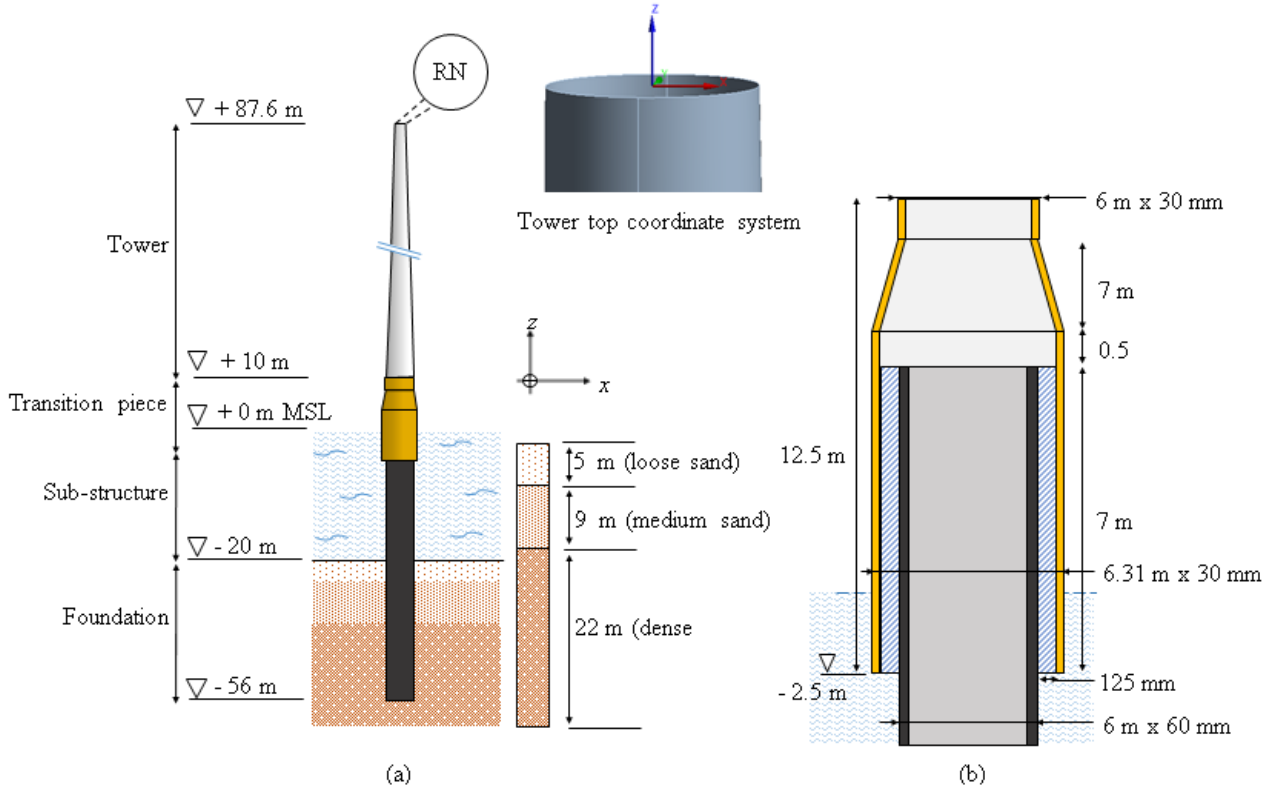
Figure 2. Geometry: a Representation of the adapted NREL 5MW and OC3 Monopile geometry embedded in layered sandy soil, b details of the transition piece adapted geometry
