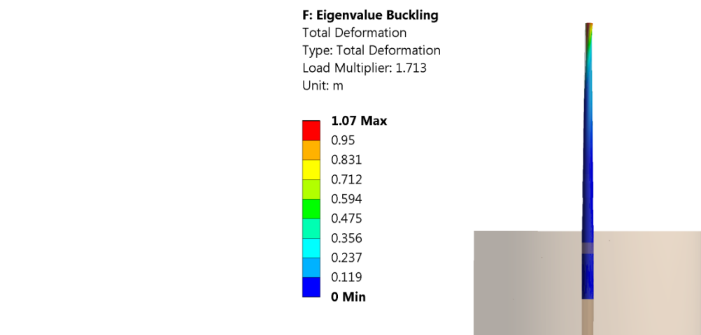
761 762 Figure 17. Buckling load multiplier and buckling mode shape of OWT support structure under ultimate load case
