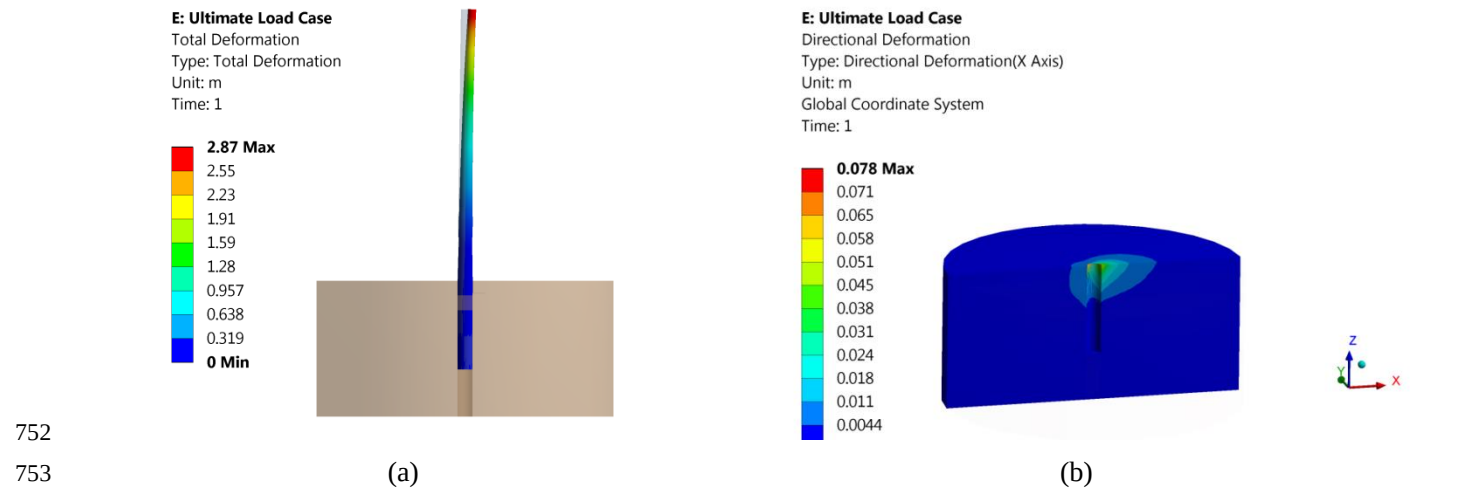
752 753 Figure 16. Deformation: a deformation of support structure, b section view of deformation of foundation and soil
