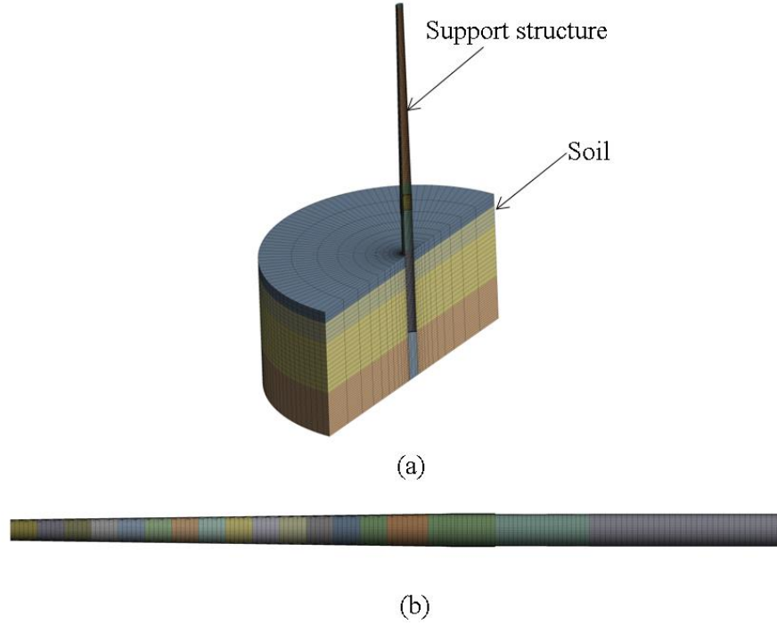
Figure 6. Mesh : a Cut view of the mesh of the assembly model, b mesh of the support structure
