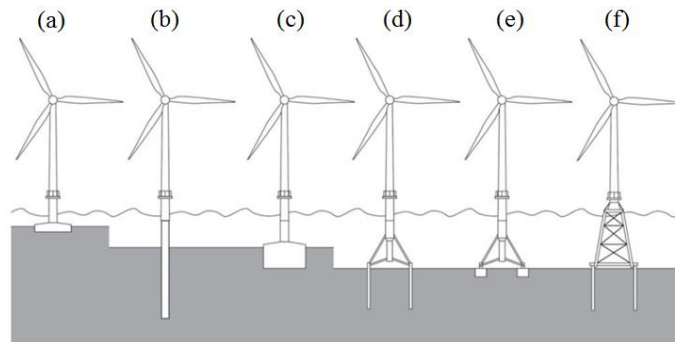
Figure 1. Typical foundation concepts [13]: a gravity-based foundation, b monopile foundation, c caisson foundation, d multi-pile foundation, e multi-caisson foundation, f jacket foundation
