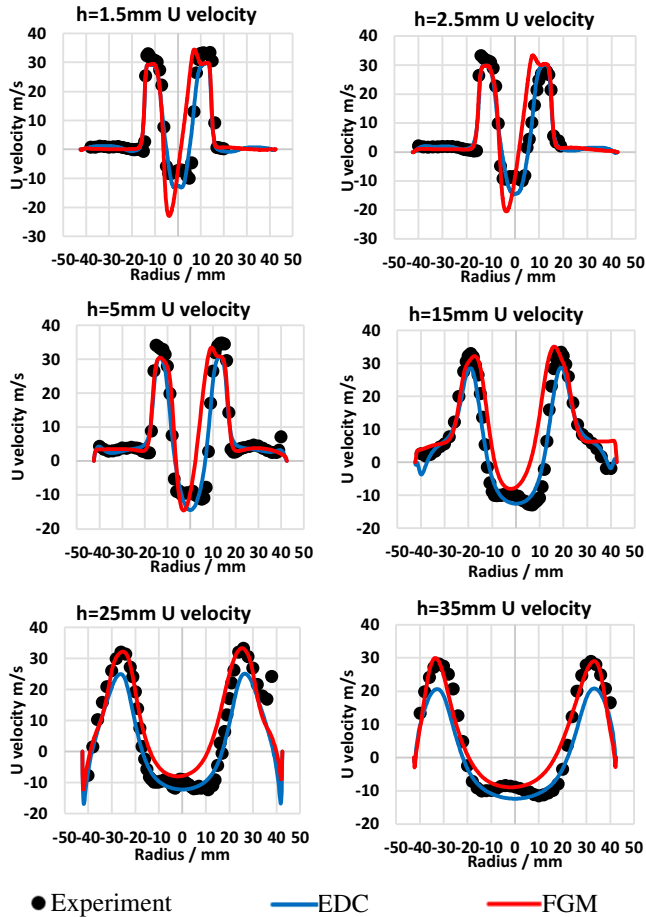
Figure 17. Axial velocity U profiles at 1bar 27kW
