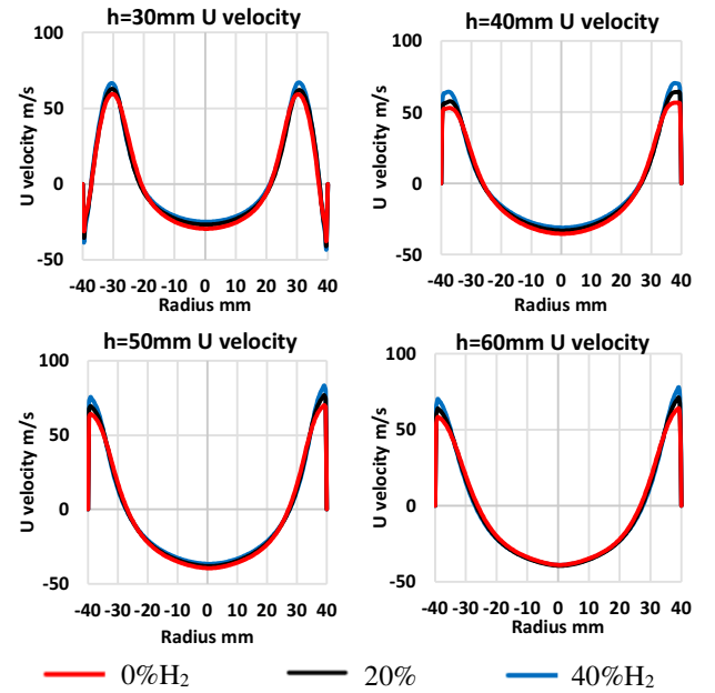
Figure 23. Axial velocity at different downstream locations with different CH 4 /H 2 blends
