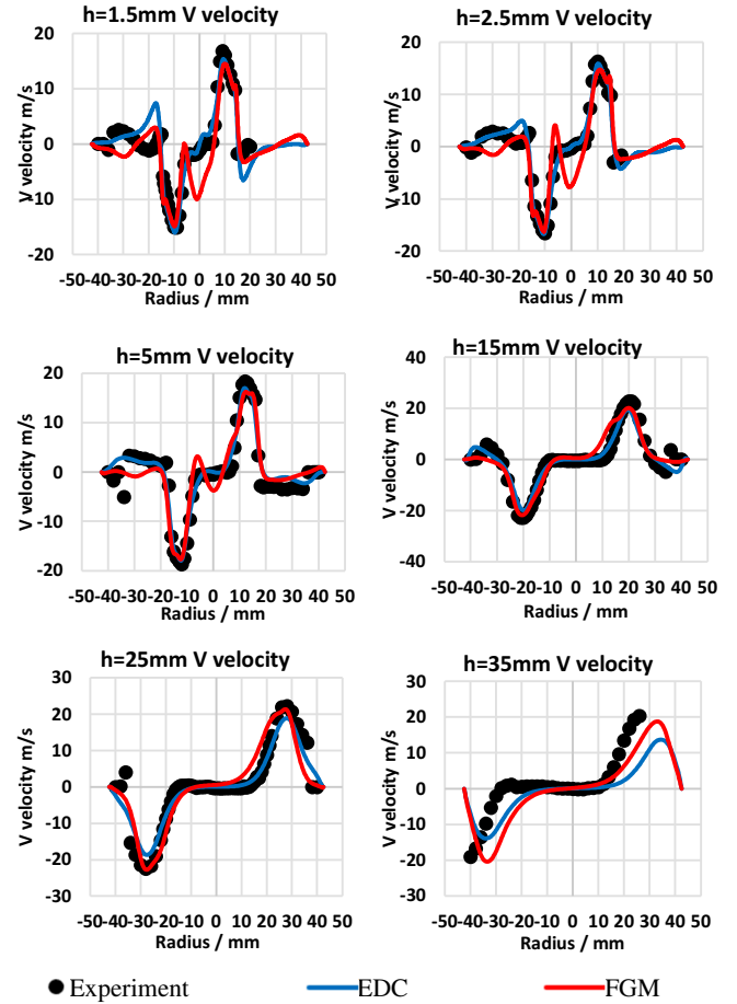
Figure C1. Low pressure burner radial velocity V at 1bar 27kW for CFD models and experiment
