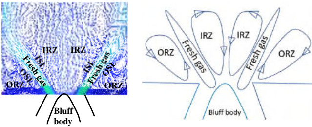
Figure 5. Schematic of swirl-stabilized flame
