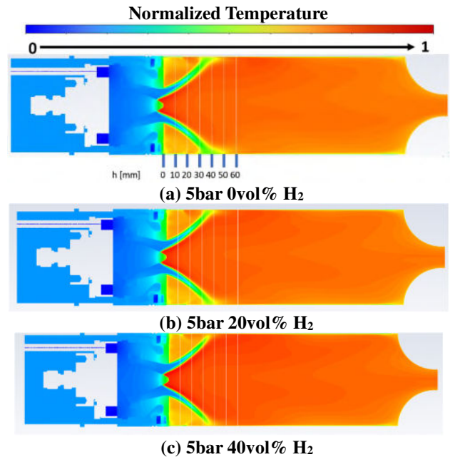
Figure 19. Contours of temperature at different \text{CH}_4/\text{H}_2 blends
