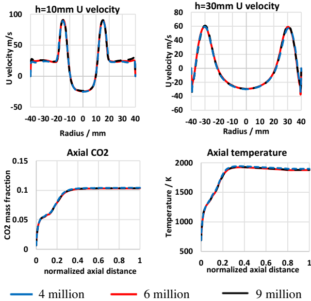
Figure A1. Grid independence study on velocity, CO 2 mass fraction temperature in the axial plane
