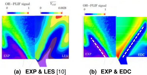
Figure 12. Time-averaged OH*-PLIF signals and OH mass fraction at 1bar 30kW
