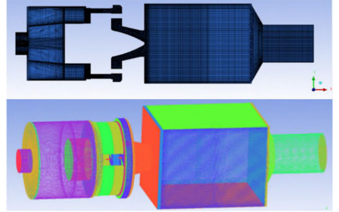
Figure 6. Grid for low-pressure burner
