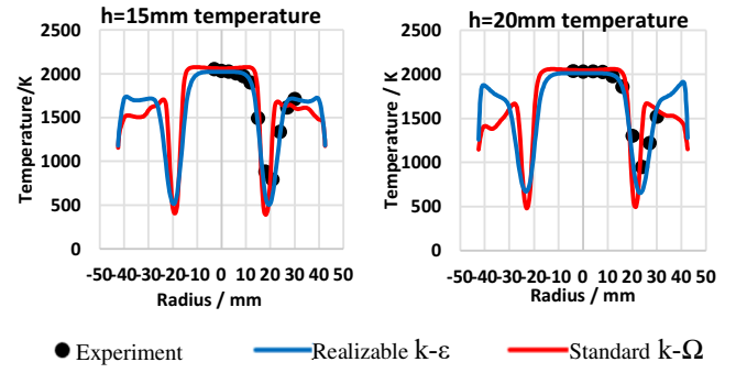
Figure B1. Temperature profiles of low pressure burner for turbulence models and experimental data at 1bar 30kW using EDC
