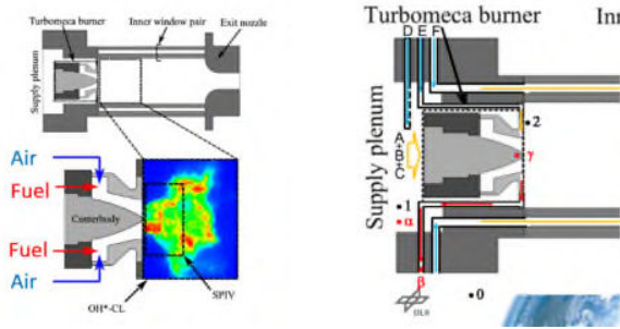
Figure 4. Schematic of higher-pressure PRECCINSTA burner [15]
