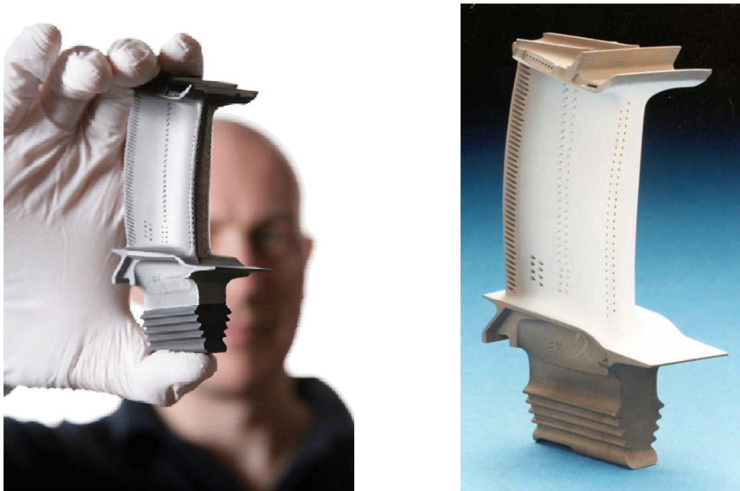
Figure 2. Rolls-Royce jet turbine blade with (a) ceramic coating (white) and (b) outlets for cooling air.
