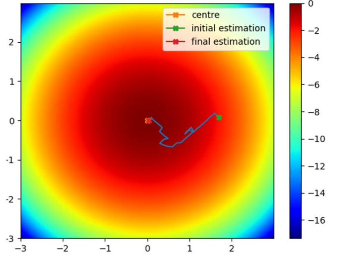
Fig. 3. Trajectory example from TD3-RNN
