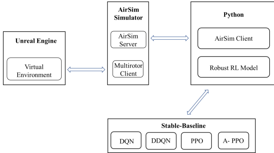
Fig. 4: Unreal Engine/Airsim/Python System Architecture
