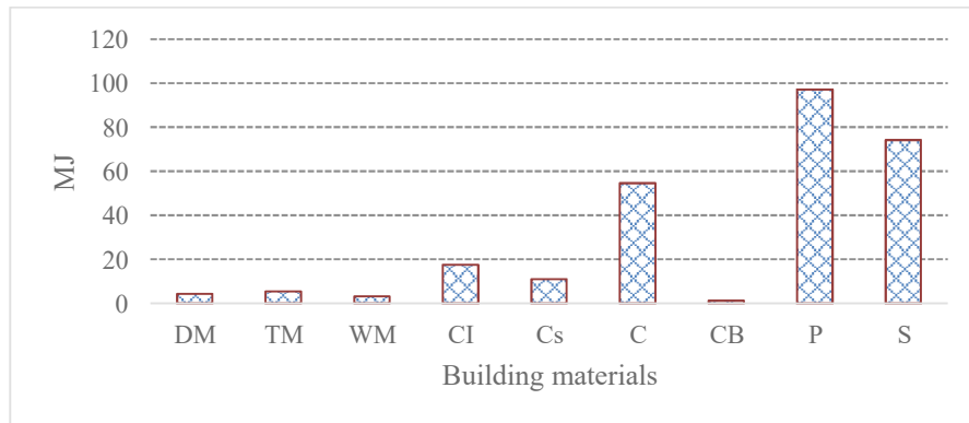
Fig 5. Energy demand where DM- Dry Mix, TM- Teclite Mix, WM-Wet Mix, CI-Cast Iron, Cs- Ceramics, C- Clay, CB-Concrete Block, P- Polypropylene and S-Steel
