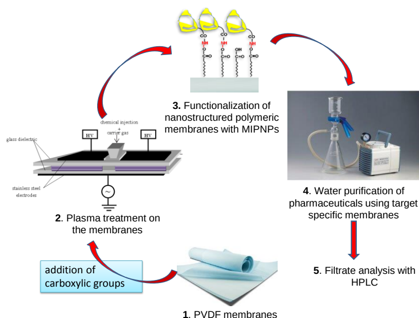
Scheme 1. Development of functionalized nanostructured polymeric membranes for water purification of pharmaceuticals using target specific membranes.
