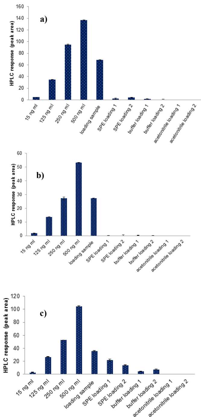
Fig 2. Diclofenac (a), metoprolol (b) and vancomycin (c) concentrations determined by HPLC in standards and before and after SPE application. Loading sample represents the starting solution of each pharmaceutical.
