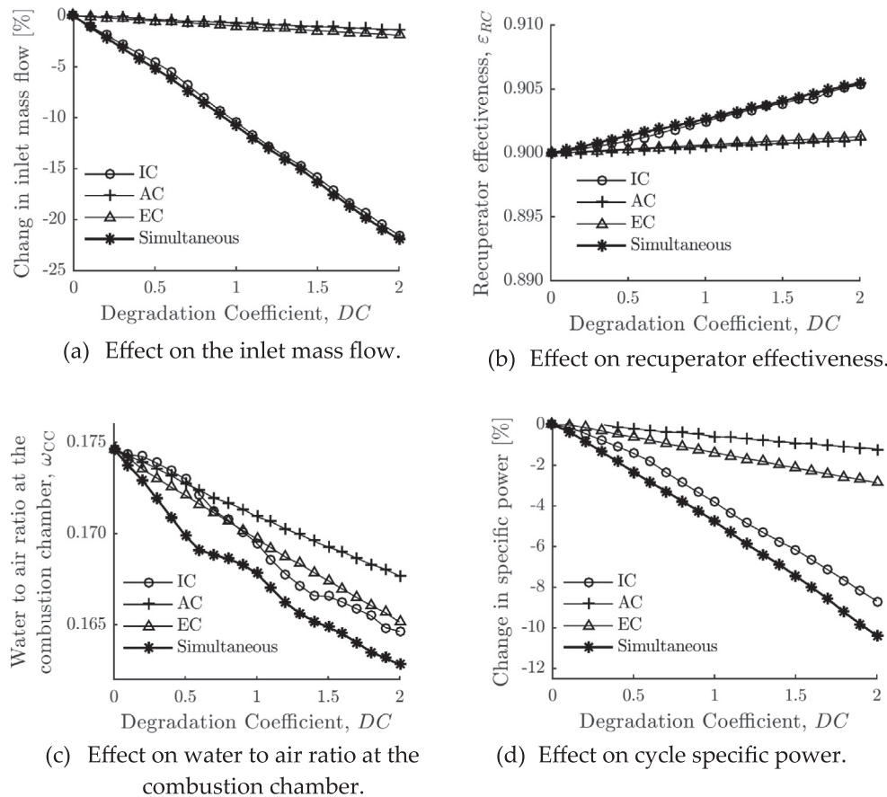
Fig. 6. Effect of the heat exchanger degradation on the (a) inlet mass flow, (b) recuperator effectiveness, (c) water to air ratio and (d) specific power. Average heat exchanger effectiveness design scenario.
