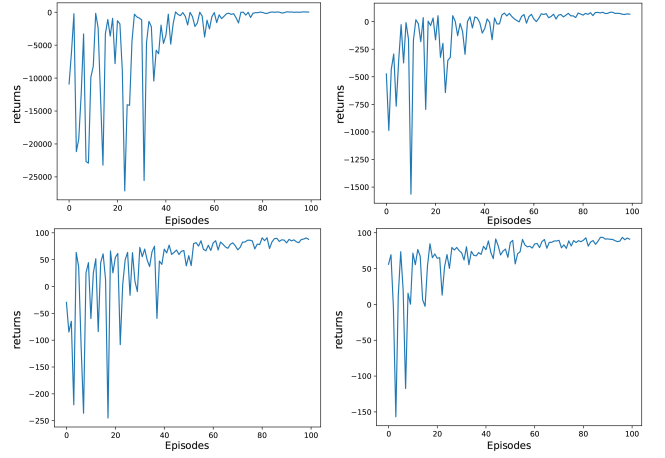
Fig. 6. This figure shows the training process of the Rossler system with different parameters, c = 0.04, 0.05, 0.06, 0.07 .
