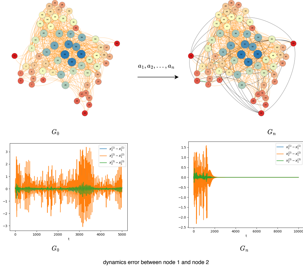
Fig. 8. This figure shows the synchronization process of cat's brain network. In the initial network G_0 and G_n edges of orange color are original edges. Black edges represent new edges added to the network and green edges represent edges which have been removed from the network. In the initial network, nodes cannot achieve the same state, x_i - x_j \neq 0 . After rewiring the network according to the action sequence obtained from our method, all nodes in the network synchronize to the state, x_i - x_j = 0 .
