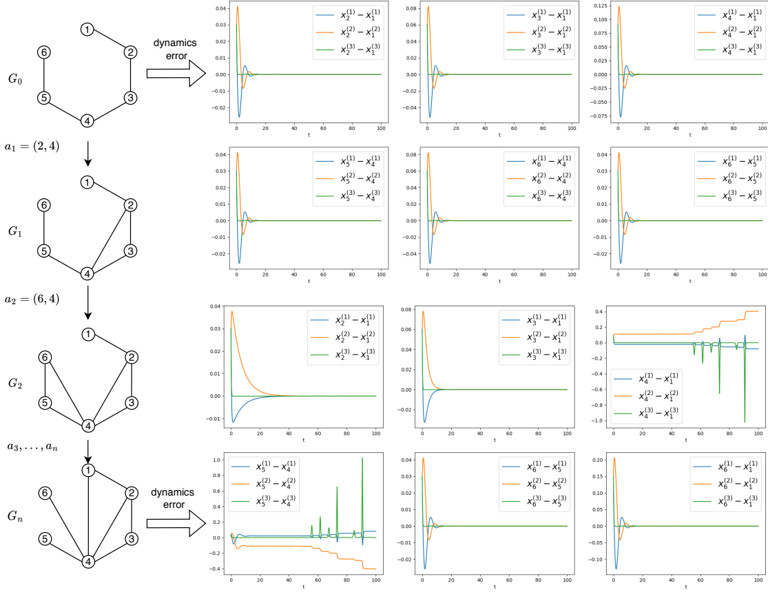
Fig. 9. This figure shows the process of cluster synchronization. Our goal is to enable nodes 1, 2, 3, 5, 6 group into a cluster and synchronize to the same state. Node 4 forms a cluster alone and achieves a different state from the first cluster. In the initial network G_0 , all nodes synchronize to the same state. After several actions by our method, a new network G_n is constructed. Nodes 1, 2, 3, 5, 6 in this complex network synchronize to the same state but node 4 achieves to a different state.
