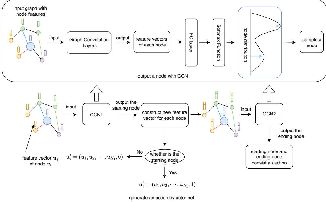
Fig. 3. This figure shows the structure of the actor net. The actor net consists of 2 GCN. The first GCN generates the starting node according to the input adjacency matrix of complex network and the feature vector \mathbf{u}_i of each node. The Second GCN generates the ending node according to the adjacency matrix and the new feature vector of each node \mathbf{u}'_i . The new feature vector \mathbf{u}'_i = (u_1, u_2, \dots, u_{N_1}, u_{N_1+1}) . u_{N_1+1} = 1 if node i is selected as the starting node, otherwise u_{N_1+1} = 0 . The graph with node features is input to the GCN layers to get feature vectors of each node. Then the feature vectors are input to the full connection layer and softmax function to get the node distribution, which used to output a node as starting node or ending node.
