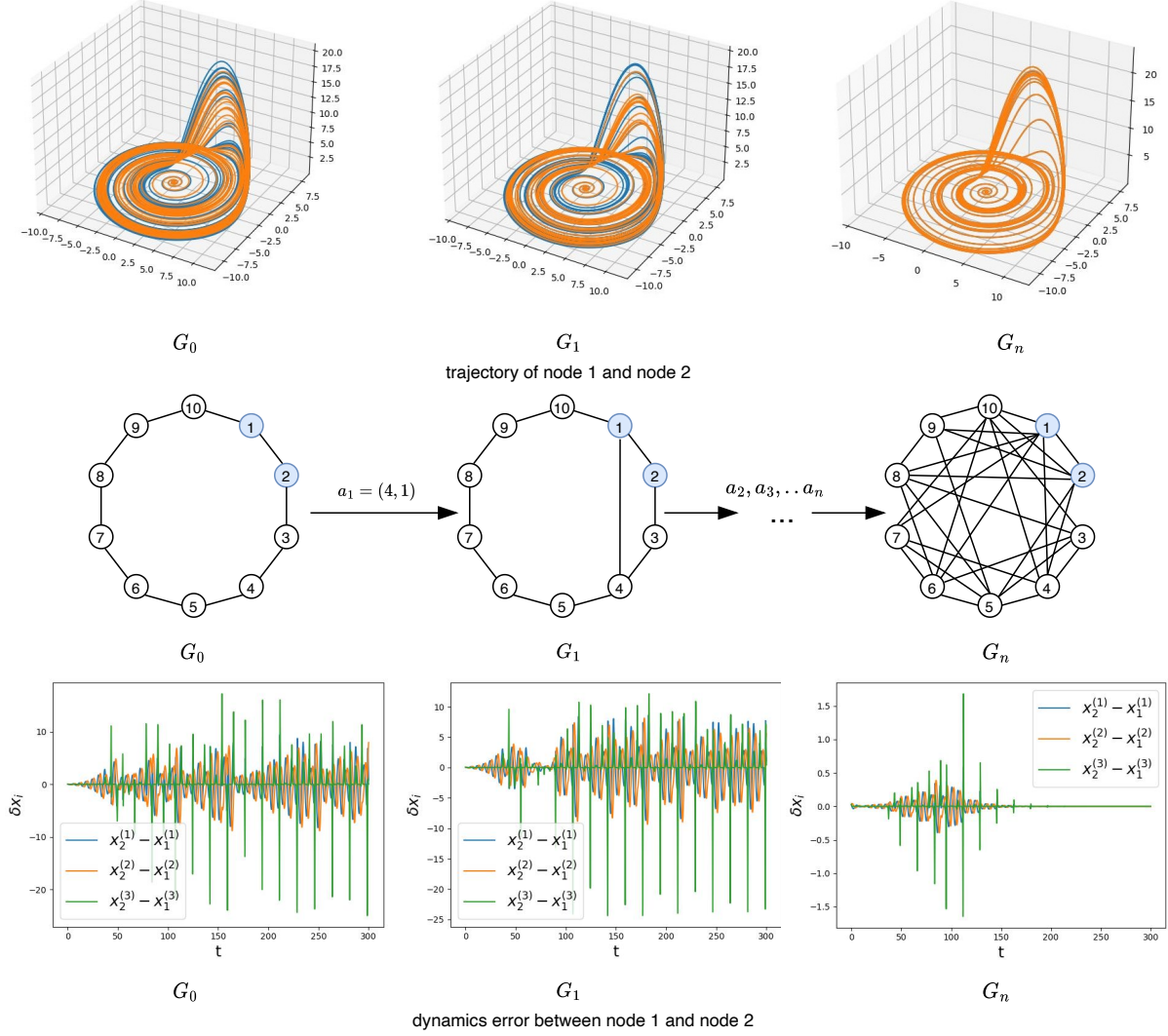
Fig. 4. This figure shows the synchronization process of nodes after several actions to the network. Nodes in the initial network G_0 do not satisfy x_i - x_j = 0 , which means they cannot synchronize to the state. Then the two Actor Nets output starting node and ending node to form the action a_1 = (4, 1) . The edge (4, 1) is added to the network G_0 according to the action and forms a new network G_1 . In this state, nodes in G_1 still do not synchronize, and the Actor Nets continue to output actions a_2, a_3, \dots, a_n to the network. The Actor Nets stop outputting actions until all the nodes in network G_n satisfy x_i - x_j = 0 , which means all nodes synchronize.
