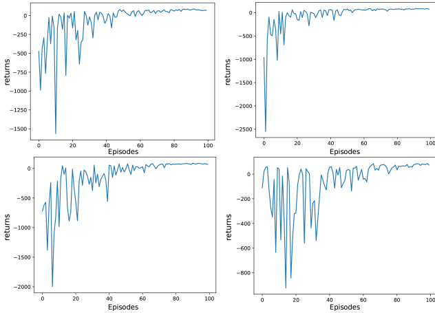
Fig. 5. This figure shows the training process of the Rossler system with different initial network structures.
