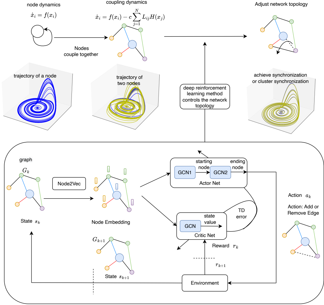
Fig. 1. Graph construction or optimization by the actor-critic graph convolutional network. In a complex network consisting of nodes with nonlinear dynamics, nodes can achieve different patterns of synchronization like cluster or global synchronization by adjusting the network topology. The observable state is the input network G_k . Feature vector of each node i is obtained by Node2Vec. Input adjacency matrix of network and feature matrix of all nodes to Actor Net to select an edge as an action. Apply the action to G_k and obtain a new network G_{k+1} as the next state s_{k+1} . In each step, the state s_k will be inputted to the critic net to estimate the state value. This process will repeat until the network achieve synchronization. Calculate the temporal difference (TD) error according to the reward and state values to update parameters of Actor Nets and Critic Net
