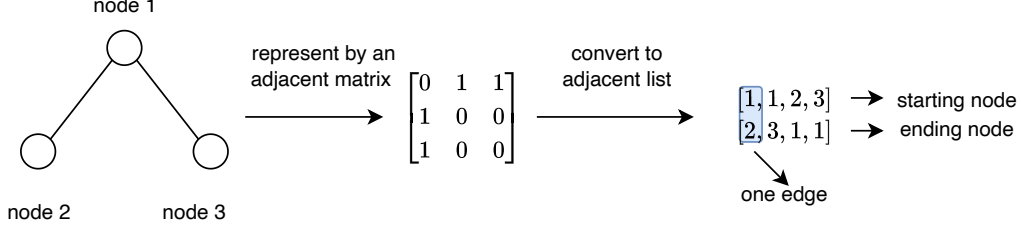
Fig. 2. Represent the adjacency matrix as an adjacency list. In adjacency list, one edge is represented by a starting node and an ending node.
