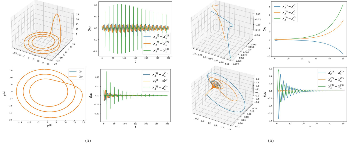
Fig. 7. (a) Alter network of Rossler system to synchronize to the limit cycle; (b) Alter network of Chua system to synchronize to the fixed point.
