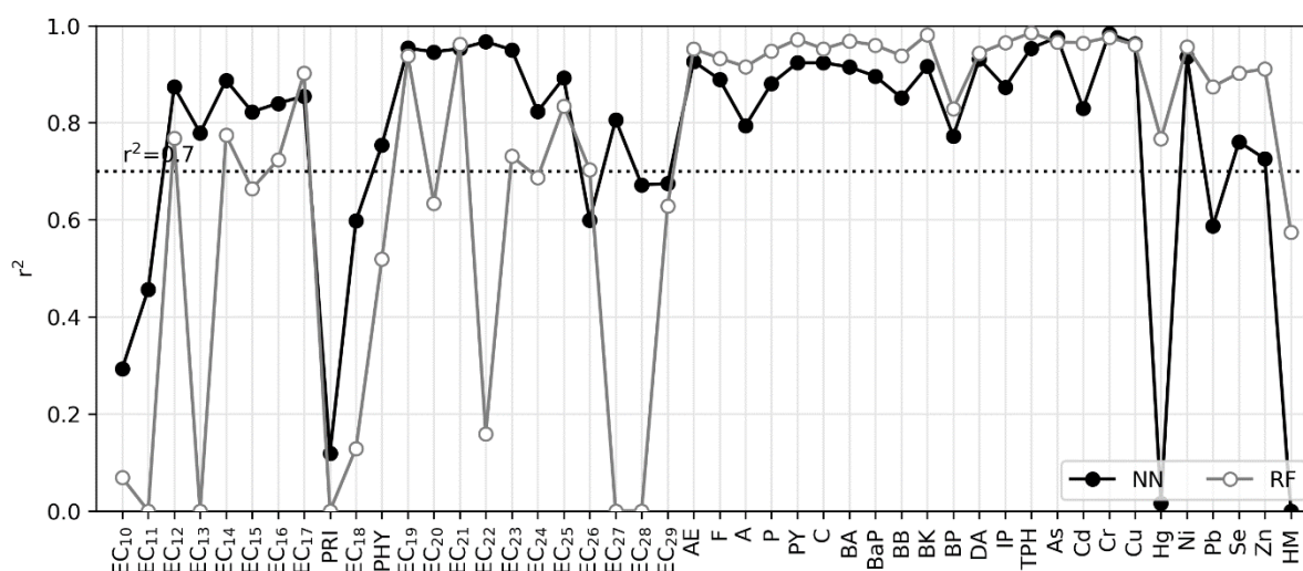
Figure 2: Prediction accuracy ( r^2 ) for the bioavailable concentration of hydrocarbons and heavy metals/metalloids using Neural Network (black) and Random Forest (grey).
