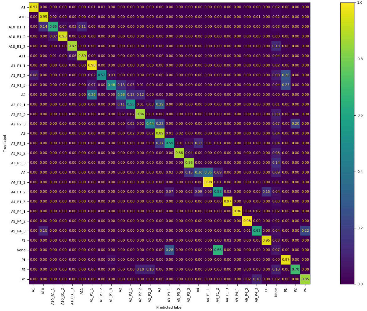
Fig. 8 Confusion matrix of the matching evaluation showing the 27 lines seen over the 95 samples of the dataset
