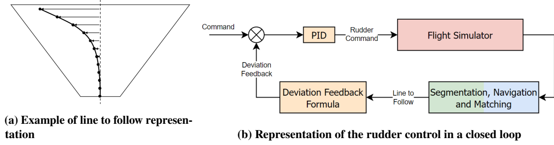
Fig. 3 Illustration diagrams for aircraft control.
