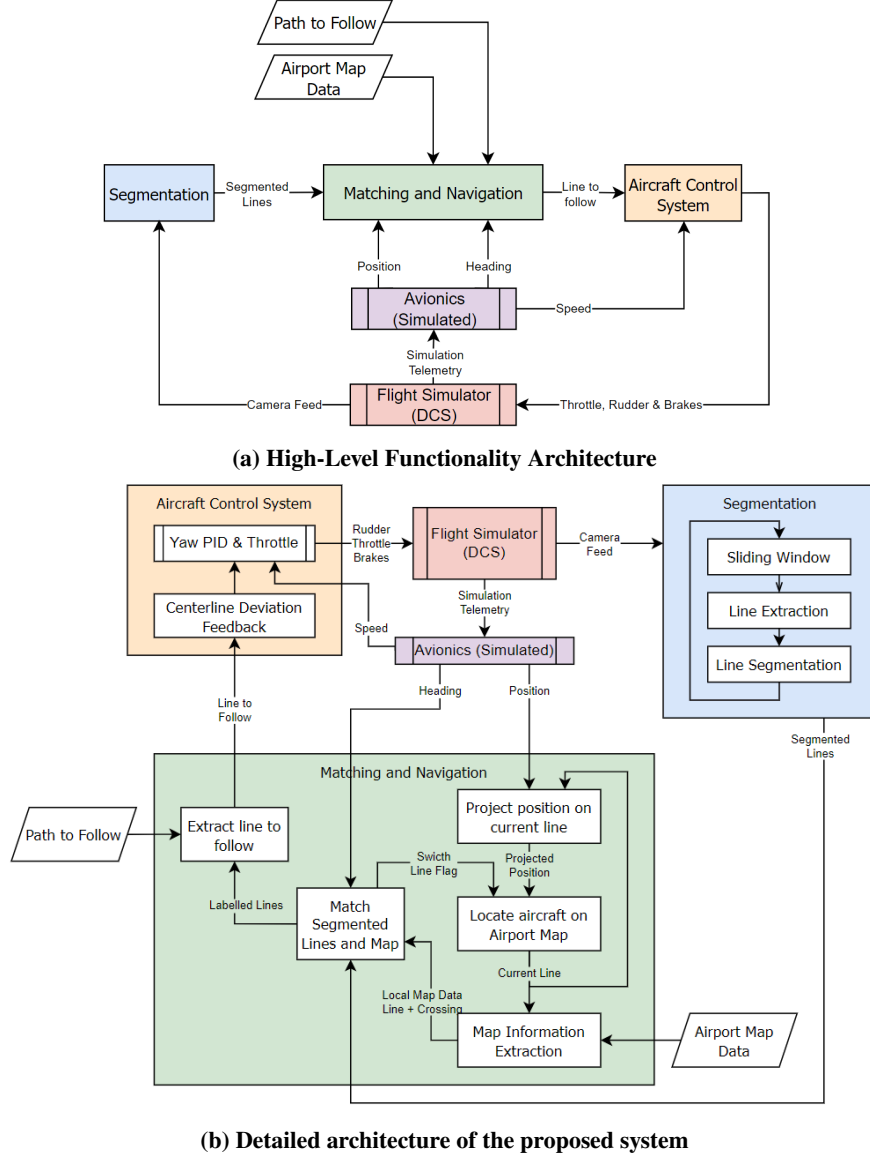
Fig. 1 Autonomous Taxiway Navigation System Architecture.
