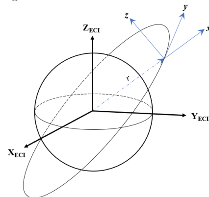
Fig. 3. LVLH coordinate system for relative motion.
