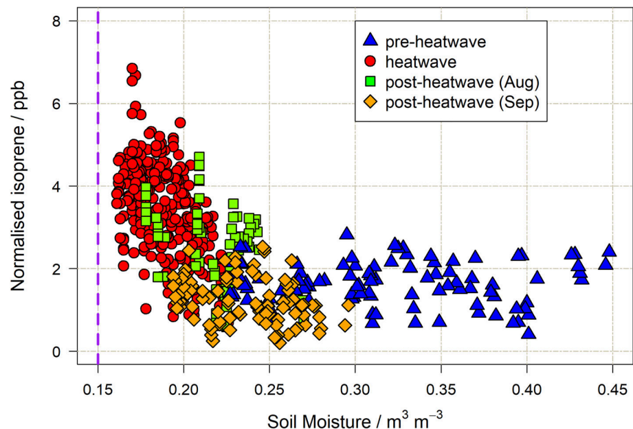
Figure 4. Correlation between normalized isoprene at the top of canopy and soil moisture. Data were filtered by PAR ( >500 \mu\text{mol m}^{-2} \text{s}^{-1} , to exclude nighttime, dawn, and dusk data) and wind speed (between 1.3 and 2.8 \text{ m s}^{-1} ). The dashed purple line at 0.15 \text{ m}^{-3} denotes the wilting point for Wytham Woods (X. Jiang et al., 2018). Isoprene mixing ratios were normalized using the G93 algorithm (Text S5 and Figure S11).
