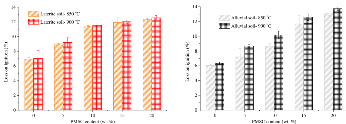
Fig. 7. Loss on ignition of PMSC mixed bricks (a) Laterite soil blended with PMSC (b) Alluvial soil blended with PMSC – both sintered at (i) 850 °C (ii) 900 °C.
