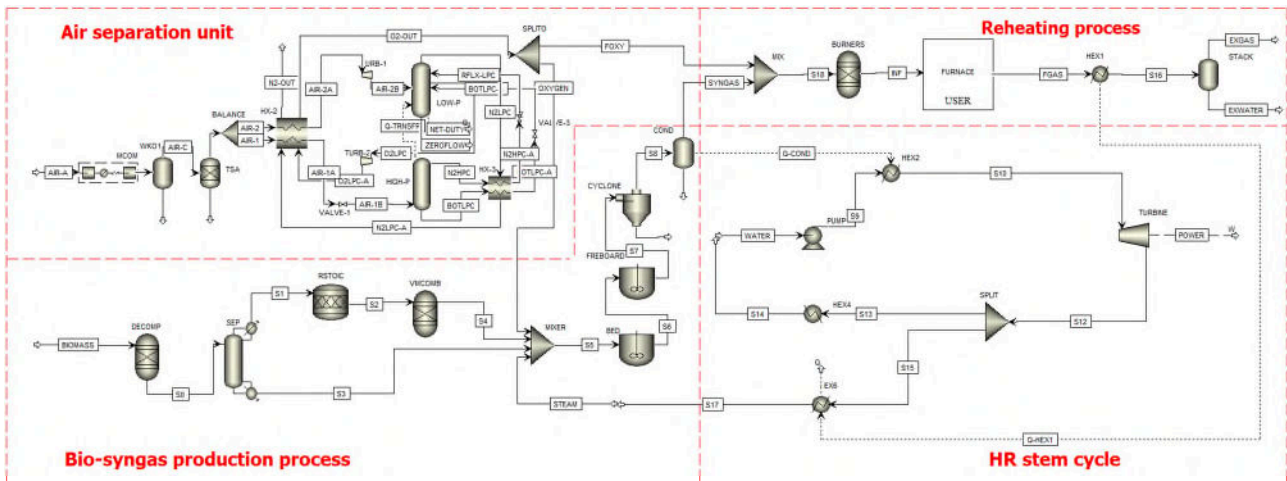
Figure 3. Process flowsheet developed using Aspen Plus
