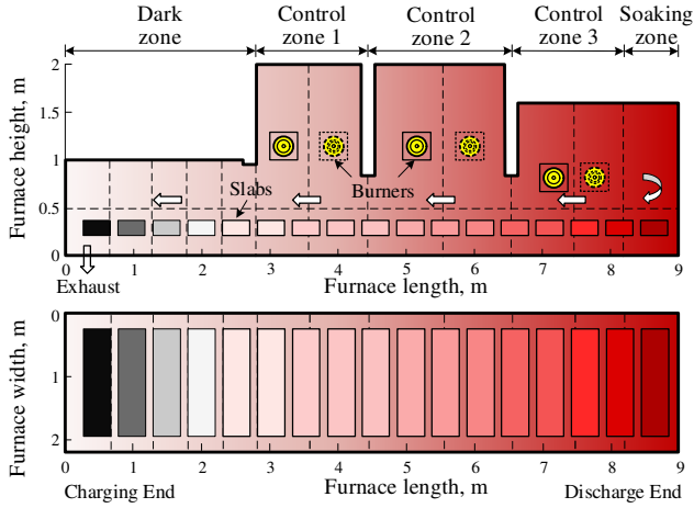
Figure 2. Outline of the pilot-scale reheating furnace
