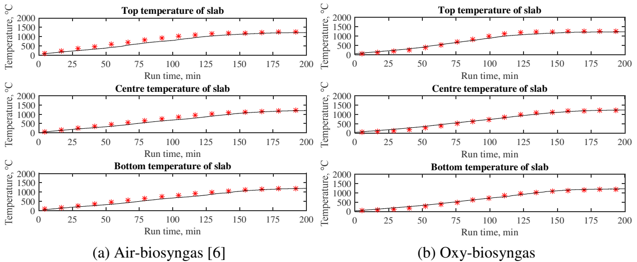
Figure 4. Comparison of the predicted slab heating profile with the desired heating profile (red symbol: predicted profile; black line: desired profile)
