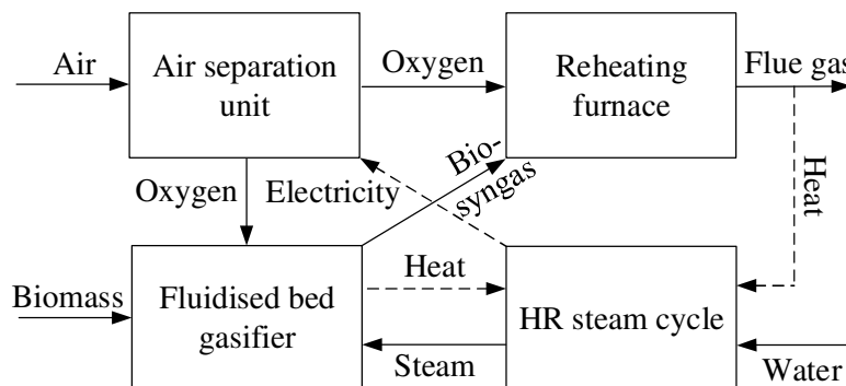
Figure 1. A schematic diagram of system integration
