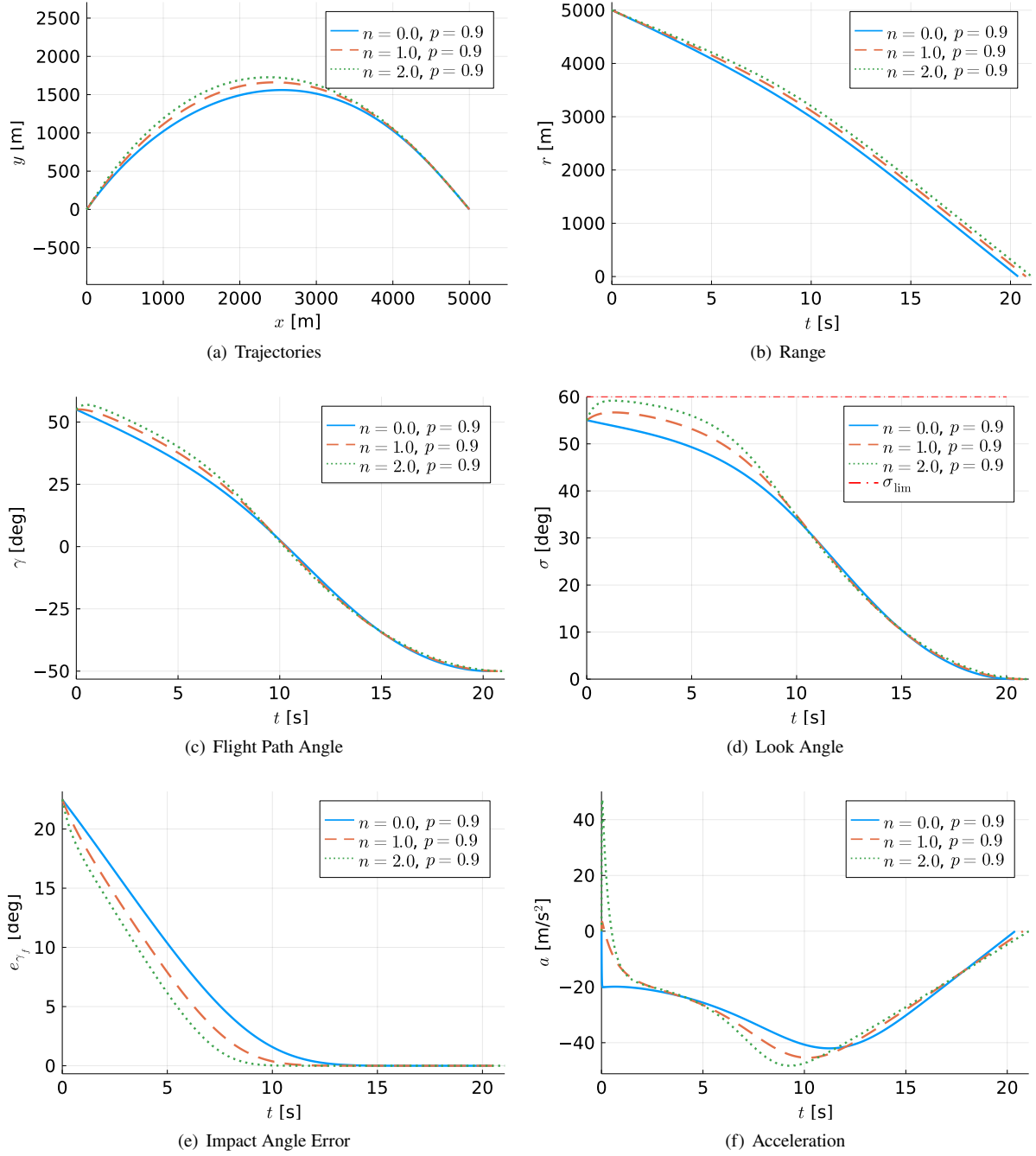
Fig. 3 Simulation Results for Case 2 - Fixed p , Various n
