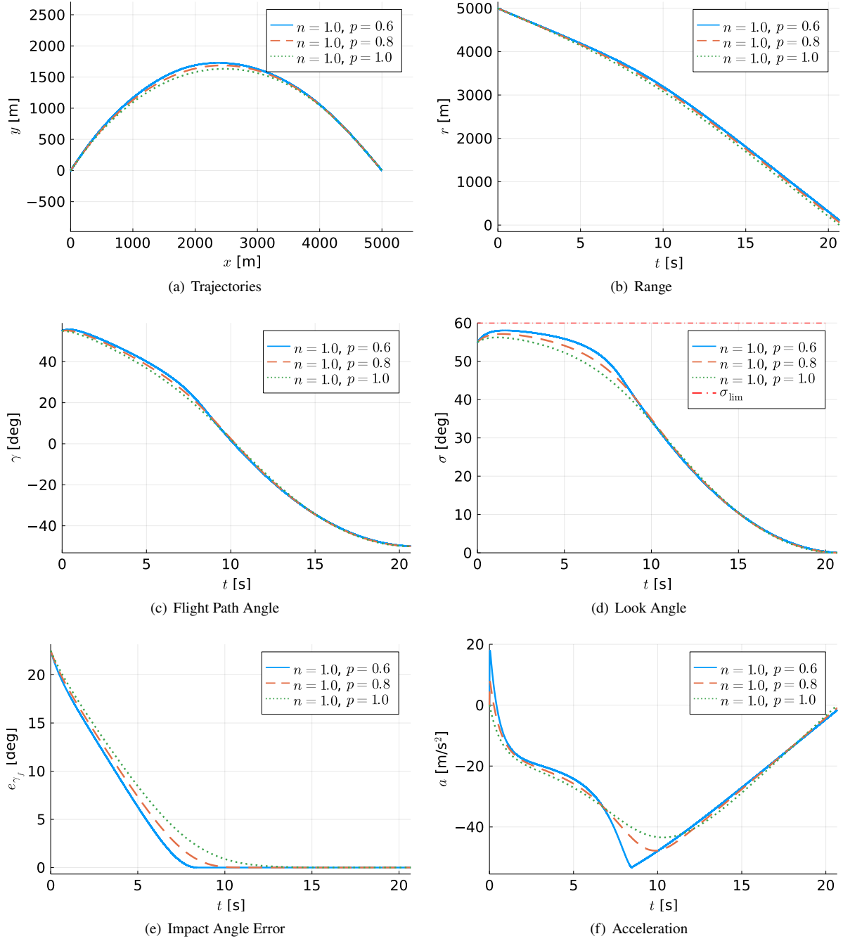
Fig. 2 Simulation Results for Case 1 - Various p , Fixed n
