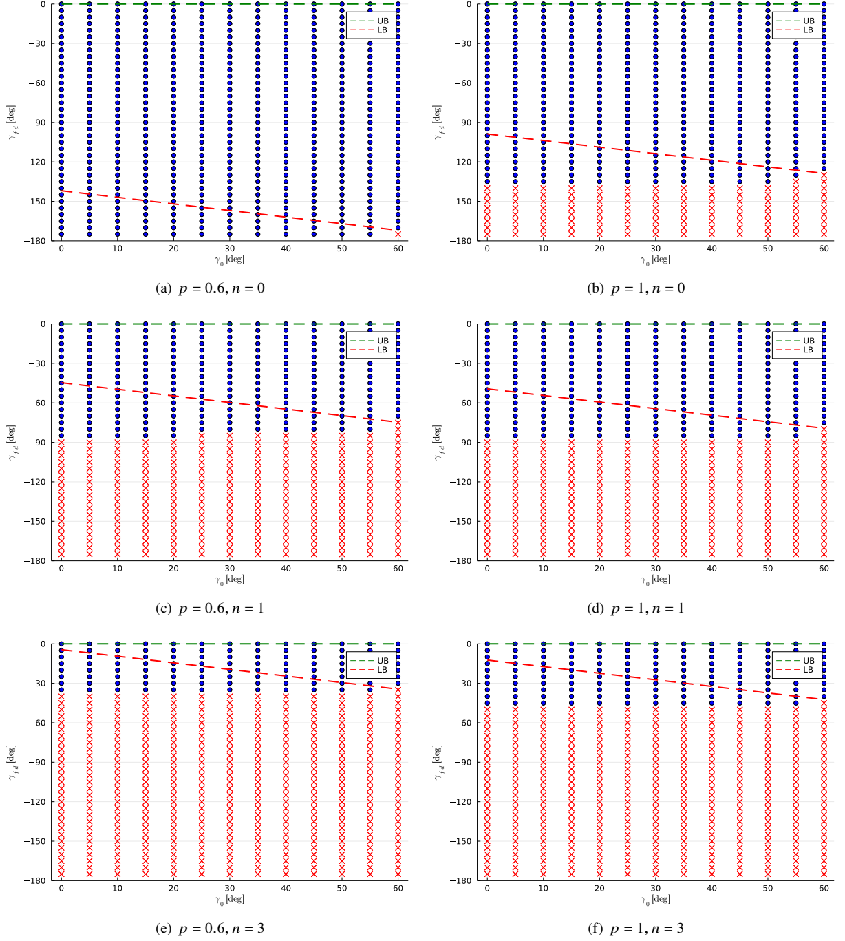
Fig. 4 Mission Accomplishment Flag and Estimated Feasible Set Boundaries for Each (\gamma_0, \gamma_{fd})
