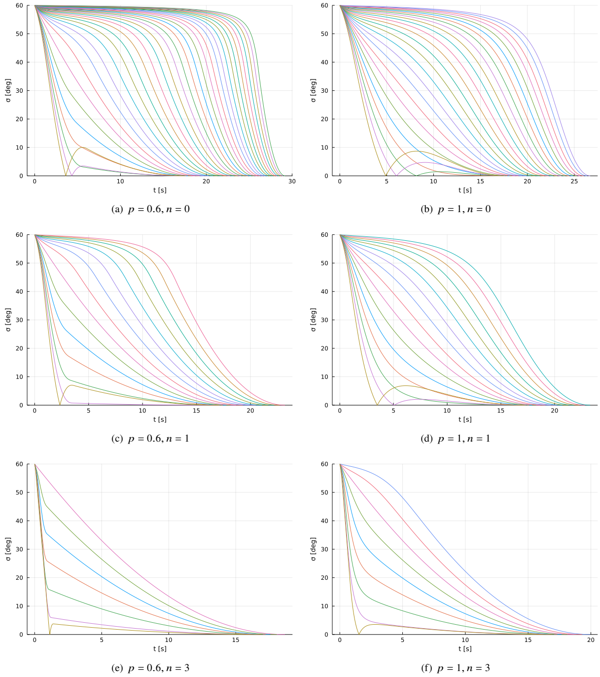
Fig. 7 Magnitude of Look Angle for \gamma_0 = \sigma_{\text{lim}}
