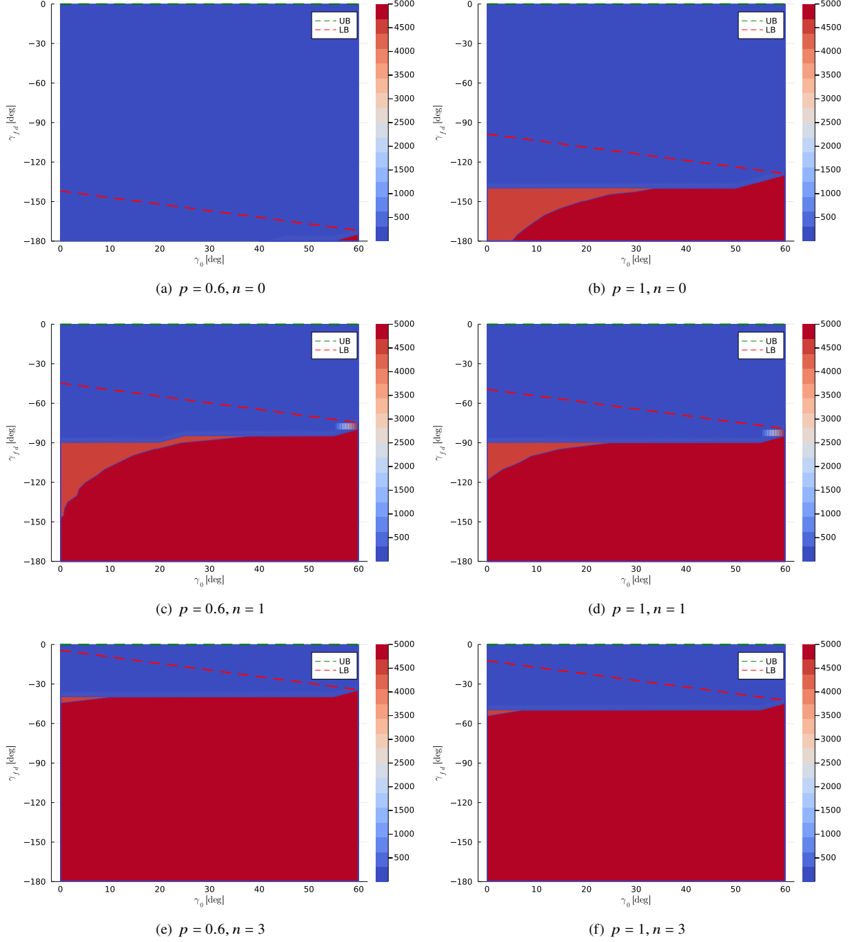
Fig. 5 Minimum Range and Estimated Feasible Set Boundaries for Each (\gamma_0, \gamma_{fd})
