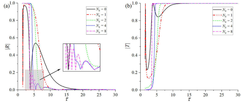
Fig. 5. The reflection and transmission coefficients versus the wave period under different numbers of internal hinges: (a). reflection coefficients; (b). transmission coefficients. Here, two edges at x = \pm d are free, N_a = N_c = 0 .
