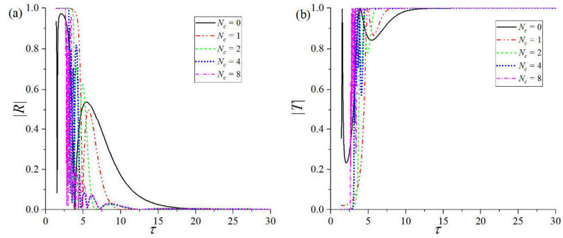
Fig. 8. The reflection and transmission coefficients versus the wave period under different numbers of internal free edges: (a). reflection coefficients; (b). transmission coefficients. Here, two edges at x = \pm d are free, N_a = N_b = 0 .
