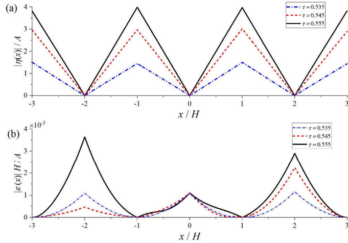
Fig. 12. Deflection (a) and distribution of the principal strain (b) of the elastic plate. Two edges at
