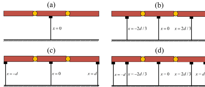
512 Fig. 10. Four different schemes to arrange pinned supports. (a) a_1 = 0 ; (b) a_1 = -\frac{2d}{3} , a_2 = 0 ,
