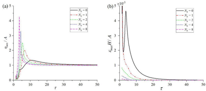
Fig. 6. The maximum deflection and principal strain in the elastic plates connected by one or multiple internal hinges: (a) maximum deflection; (b). maximum principal strain. Here, two edges at x = \pm d are free, N_a = N_c = 0 .
