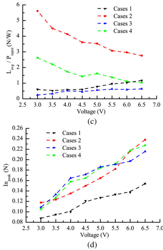
Figure 9. (a) Flapping frequency; (b) Rotary speed; (c) Lift-to-power ratio; (d) Peak values of the inertial force of the FWR in a range of input voltage.
