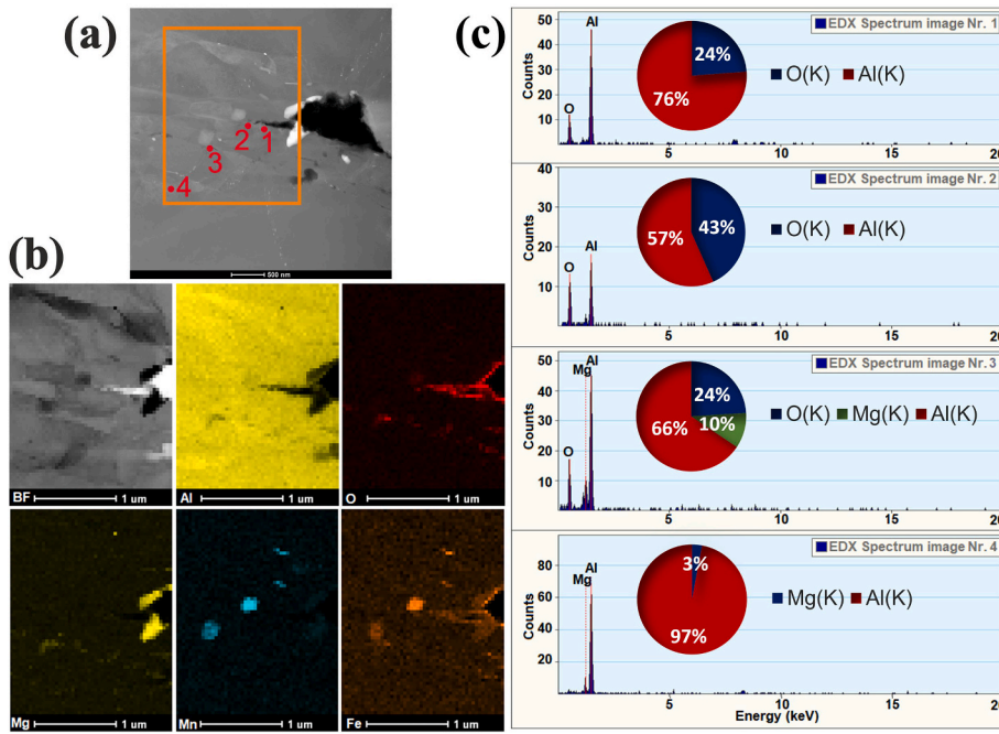
Fig. 17. Scanning transmission electron microscopy with corresponding energy dispersive X-ray spectroscopy (STEM-EDX) elemental mapping showing the spatial distribution of the oxide and intermetallics: (a) High-angle annular dark-field scanning transmission electron microscope (HAADF-STEM) overview image; (b) Bright field scanning transmission electron microscopy image with corresponding energy dispersive X-ray spectroscopy (STEM/EDX) elemental mappings of the area marked in overview (a); (c) spot analysis with energy dispersive X-ray spectroscopy (EDX) spectra marked in (a).
