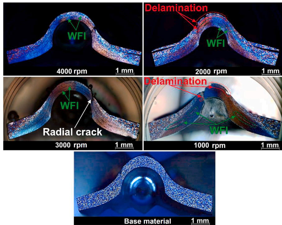
Fig. 13. Macrographs of the specimens after small punch testing prepared from welds produced with rotational speeds in the range of 1000–4000 rpm.
