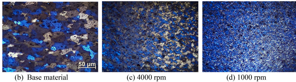
Fig. 10. Grain size distribution obtained in the weld sections shown by using cross-section polarized light microscopy for various conditions of welded samples produced at rotational speeds of 1000–4000 rpm.
