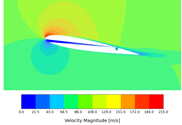
Figure 9: Velocity contour of NACA0012 attached with trapped vortex cavity connected with passive blowing tunnel at its optimal ratio of 4. The color bar represents the velocity magnitude.
