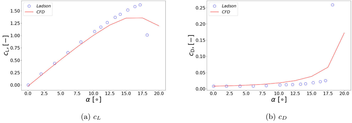
Figure 7: Simulation validation with Experimental result by Ladson [20], \alpha[^\circ] represents angle of attack, c_L[-] represents the Lift coefficient, and c_D[-] represents the Drag coefficient
