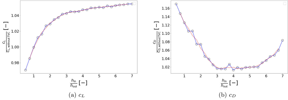
Figure 11: NACA0012 attached with TVC connected to passive blowing tunnel: h_{in}/h_{out} [-] represents the length ratio between the channel inlet and channel outlet; c_L [-] represents Lift coefficient and c_D [-] represents Drag coefficient. The blue solid line represents results obtained from CFD while the red dashed line represents window-averaged results.
