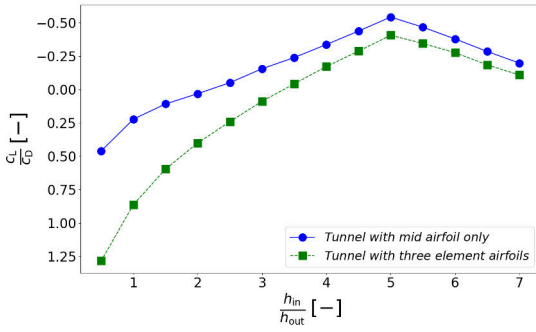
Figure 25: Comparison of tunnel performance for single mid airfoil and three-element airfoils: h_{in}/h_{out}[-] represents the length ratio between the tunnel inlet and tunnel outlet; c_L/c_D[-] represent Lift coefficient versus Drag coefficient
