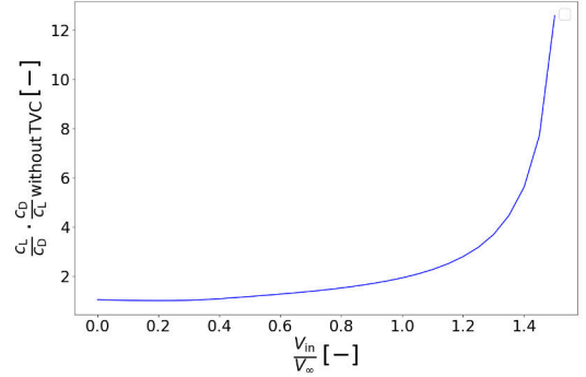
Figure 8: NACA0012 attached with TVC with mass-flow rate anchored inside the cavity: V_{\text{in}}/V_\infty[-] represents the mass-flow rate in term of velocity entering into the cavity versus free-stream velocity; c_L/c_D[-] represent Lift coefficient versus Drag coefficient
