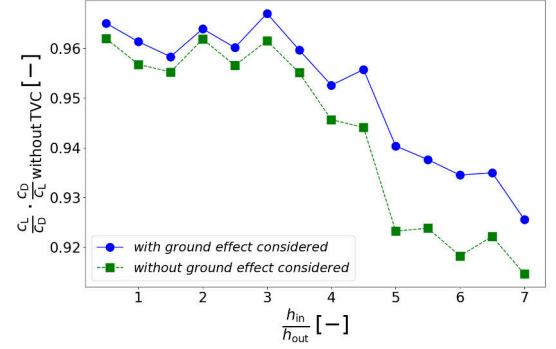
Figure 23: Comparison of three-element airfoils with TVC and internal tunnel in mid with and without ground effect considered: h_{in}/h_{out} [-] represents the length ratio between the tunnel inlet and tunnel outlet; c_L/c_D [-] represent Lift coefficient versus Drag coefficient
