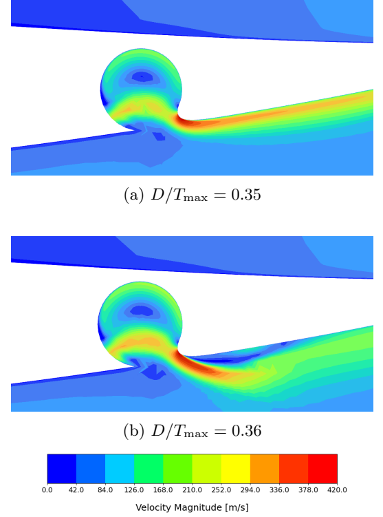
Figure 18: Velocity contours at 0.35 and 0.36 diameter-to-thickness ratios.
